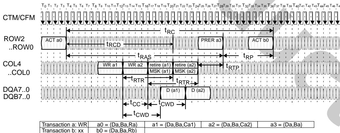
Figure 14-1 Write Transaction Example
