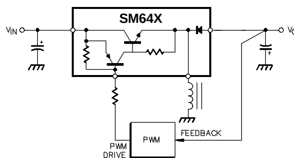
FIGURE 4 - NEGATIVE OUTPUT DOWN/UP (BUCK-BOOST) CONVERTER
