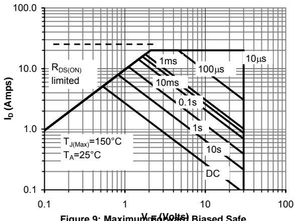
Figure 9: Maximum Safe Operating Area (Note F)
