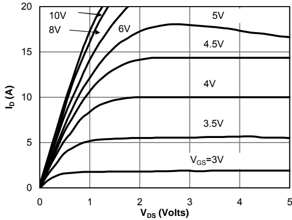
Fig 1: On-Region Characteristics
