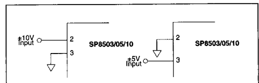
Figure 2. a) \pm 10V Range b) \pm 5V Range — Without Trims
