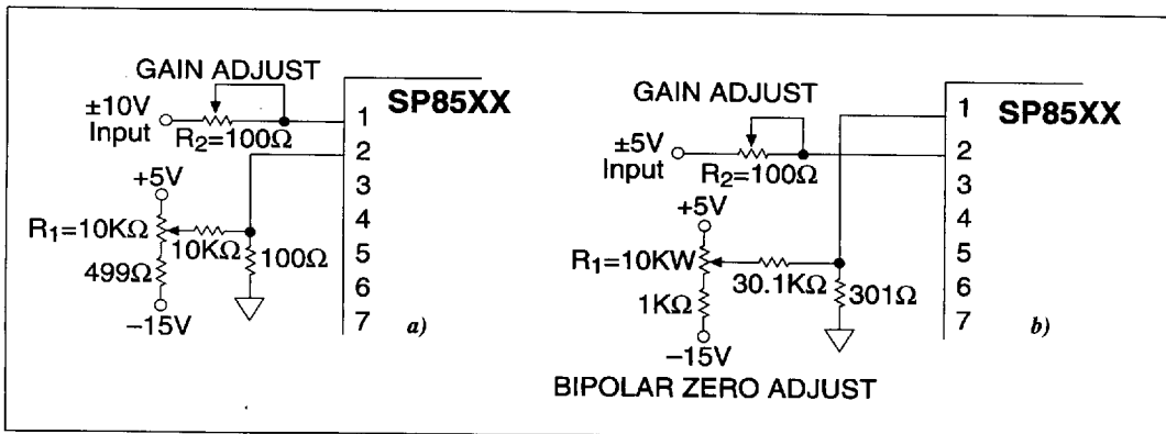
Figure 3. a) \pm 10V Range b) \pm 5V Range — With External Trims
