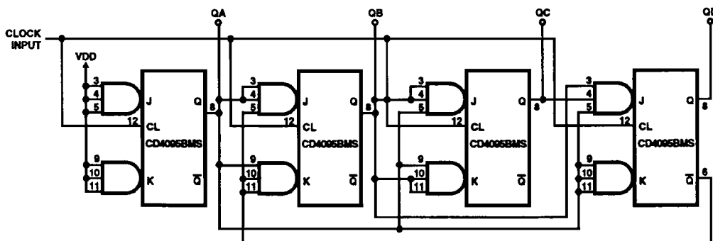
FIGURE 4. CD4095BMS CONNECTED IN TOGGLE MODE
