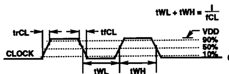
FIGURE 3. CLOCK PULSE RISE AND FALL TIME WAVEFORMS
