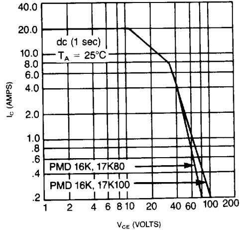
SAFE OPERATING AREA (PMD 16K, 17K SERIES)
