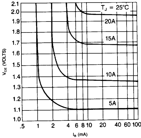
COLLECTOR SATURATION REGION (PMD 16K SERIES)
