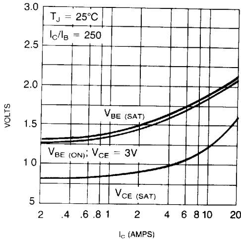
ON VOLTAGE VS COLLECTOR CURRENT (PMD 16K SERIES)
