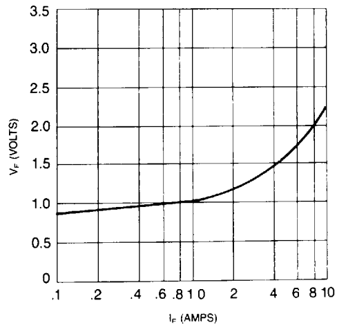
FORWARD VOLTAGE OF D1 (PMD 17K SERIES)
