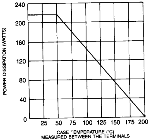
POWER DERATING (PMD 16K, 17K SERIES)
