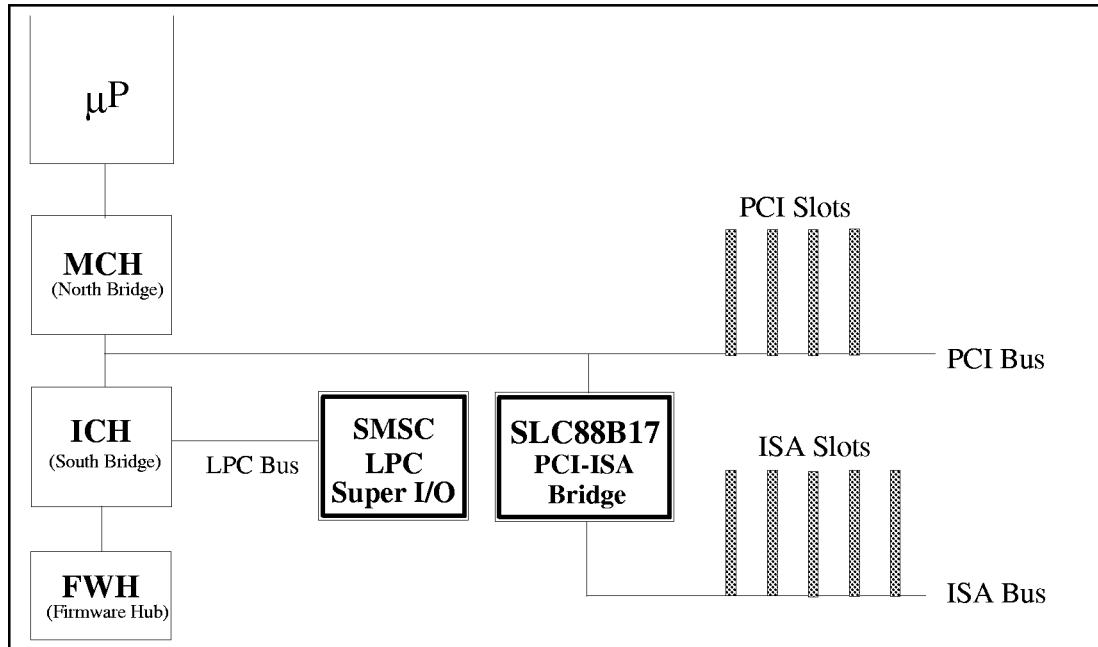
FIGURE 1 – DESKTOP APPLICATION
