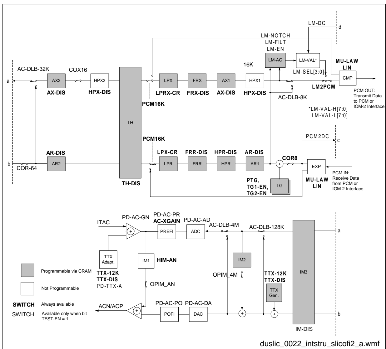
Figure 36 AC Test Loops SLICOFI-2
