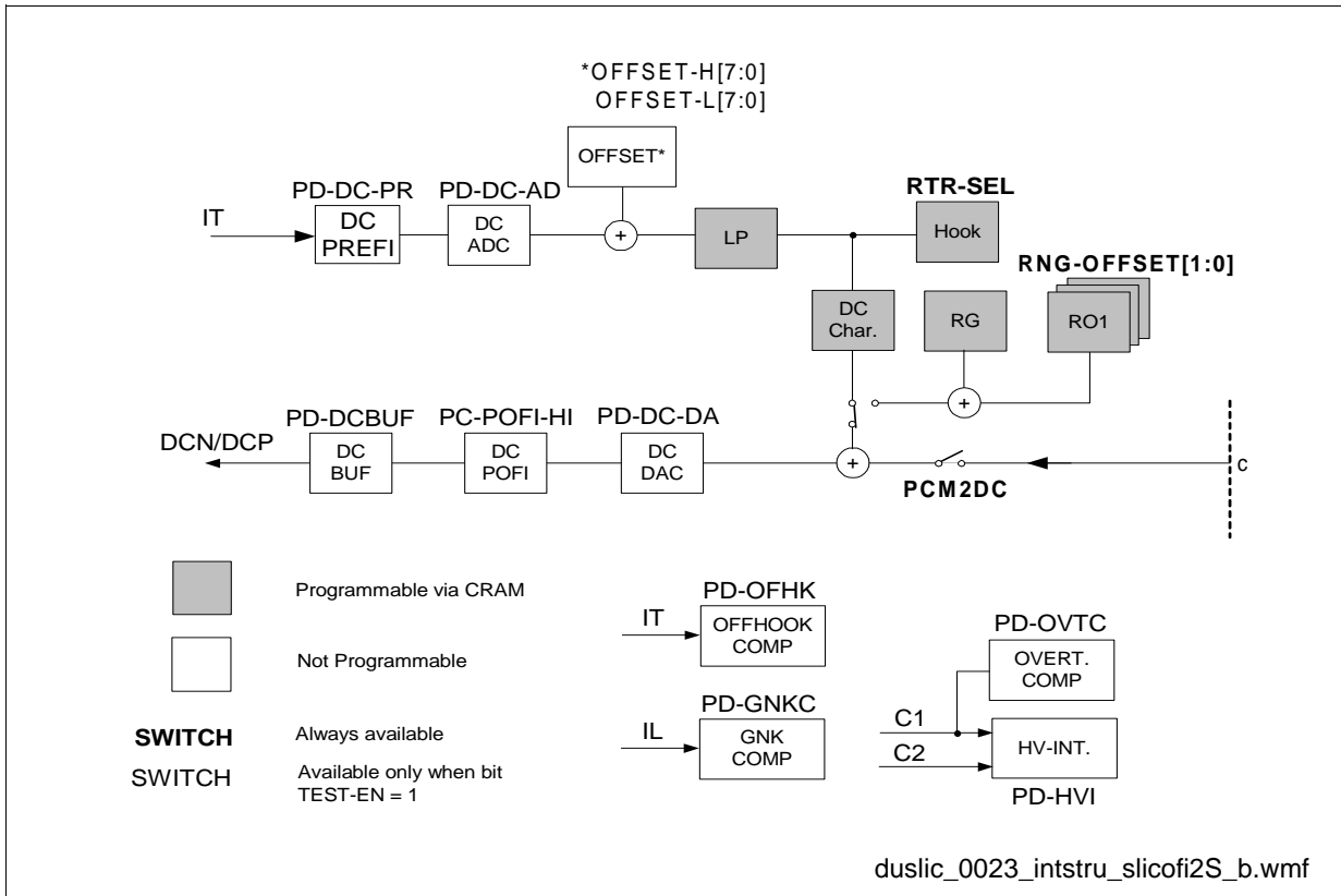
Figure 40 DC Test Loops SLICOFI-2S/-2S2
