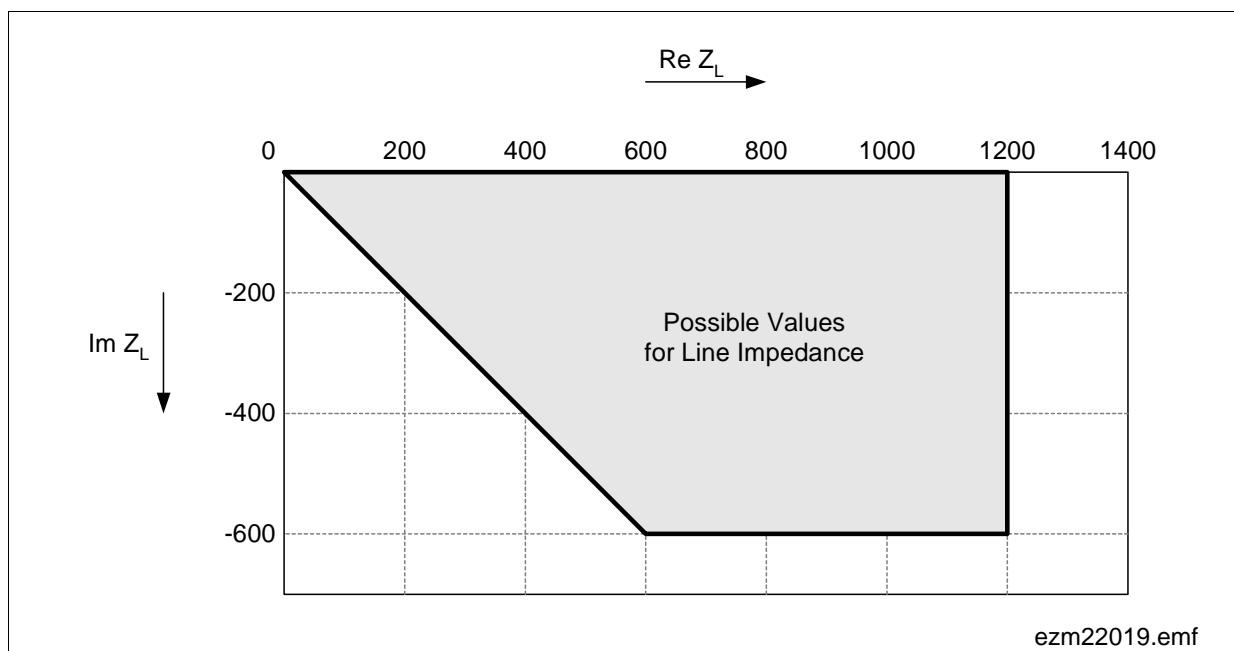
Figure 18 Nyquist Diagram
