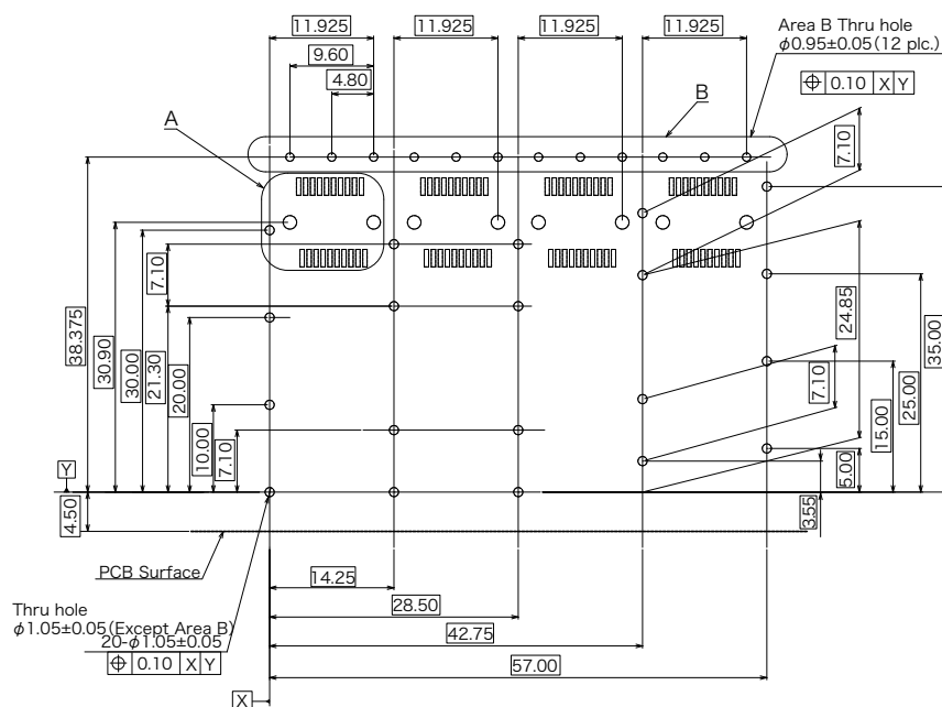
PCB Thickness : 1.60±0.19
