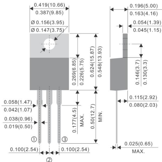
TO-220AB Dimension
