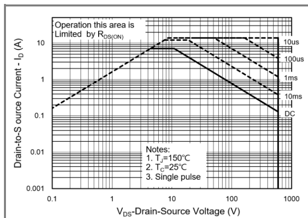
Fig.12 PJP Maximum Safe Operating Area
