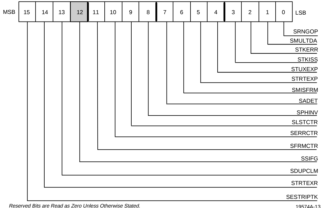
Figure 12. Status Register 2 – Lower 16 Bits (ST2L) (NPADDR = 03h)
