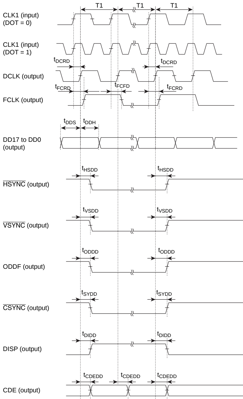
Figure 7-13 Master Mode Display Timing
