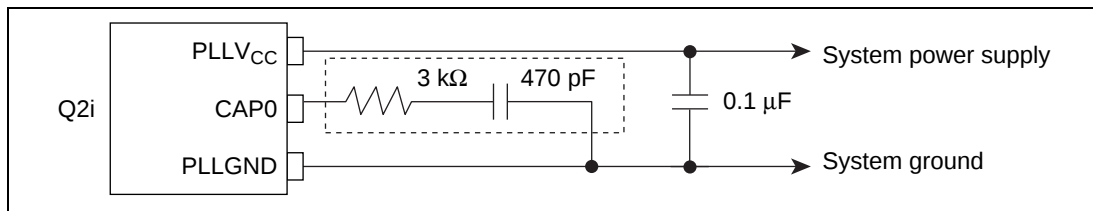
Figure 2-3 Sample CAP0 Pin Connection Circuit
