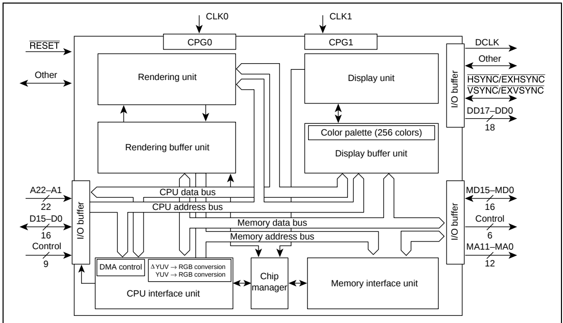
Figure 1-2 Internal Block Diagram
