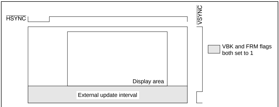
Figure 5-1 (a) External Update Interval (Interlace Mode)
