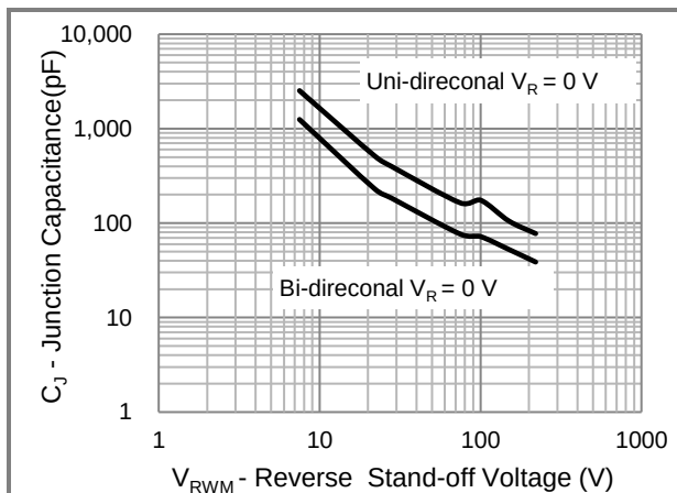
Fig.4 Typical Capacitance
