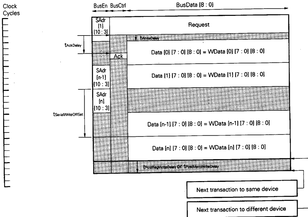
Figure 7-4. Write Transaction with Serial Address Packet
