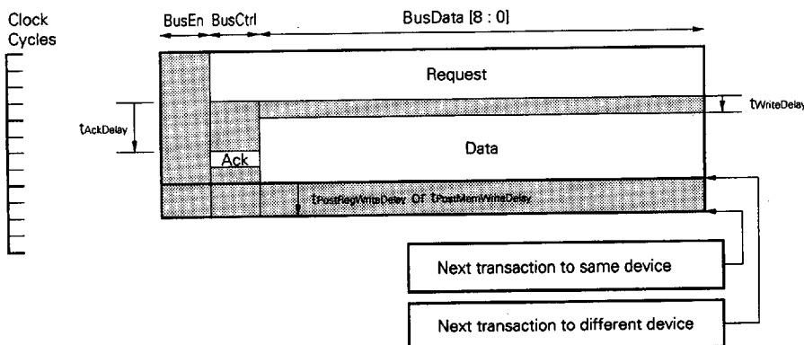
Figure 7-2. Write Transaction
