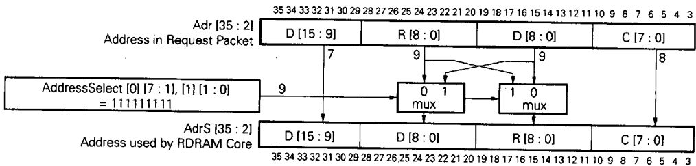
Figure 9-1. AddressMapping Hardware
