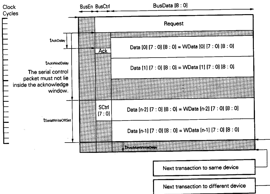
Figure 7-6. Write Transaction with Serial Control Packet
