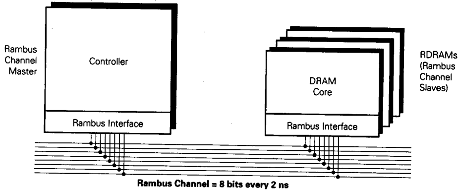
Figure 2-1. Logical Representation
