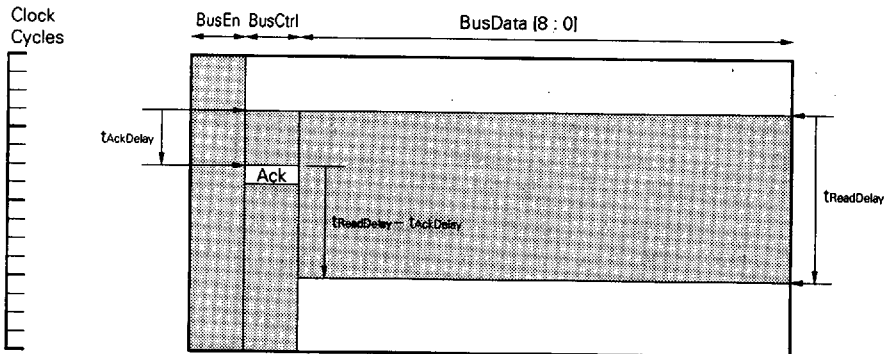
Figure 7-1. Read Transaction
