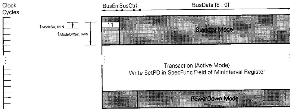
Figure 6-4. ActiveMode to PowerDownMode Transition
