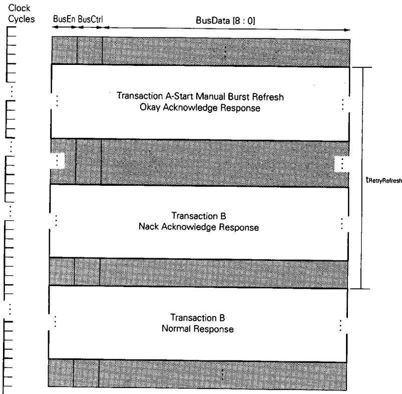
Figure 8-2. Transaction Holdoff Due to Burst Refresh
