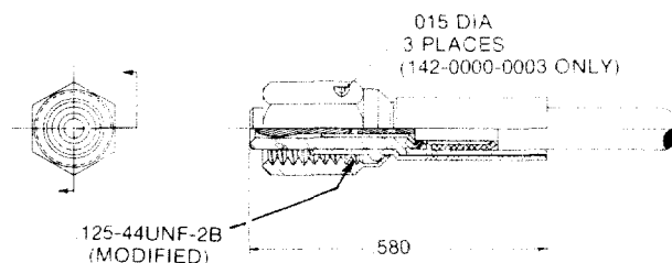
STRAIGHT PLUGS
