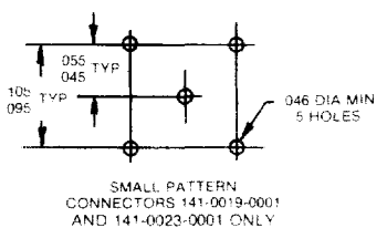
PRINTED CIRCUIT RECEPTACLE MOUNTING HOLE PATTERN
