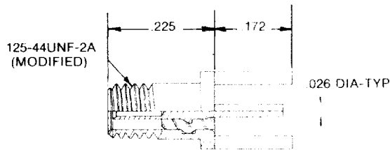
STRAIGHT PRINTED CIRCUIT RECEPTACLE 141-0004-0001
