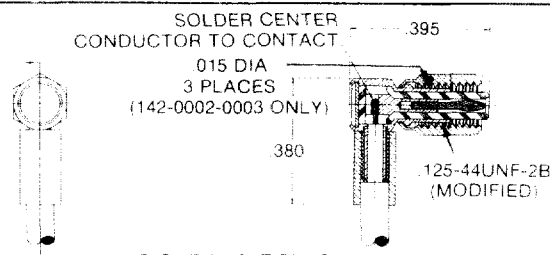
RIGHT ANGLE PLUG
