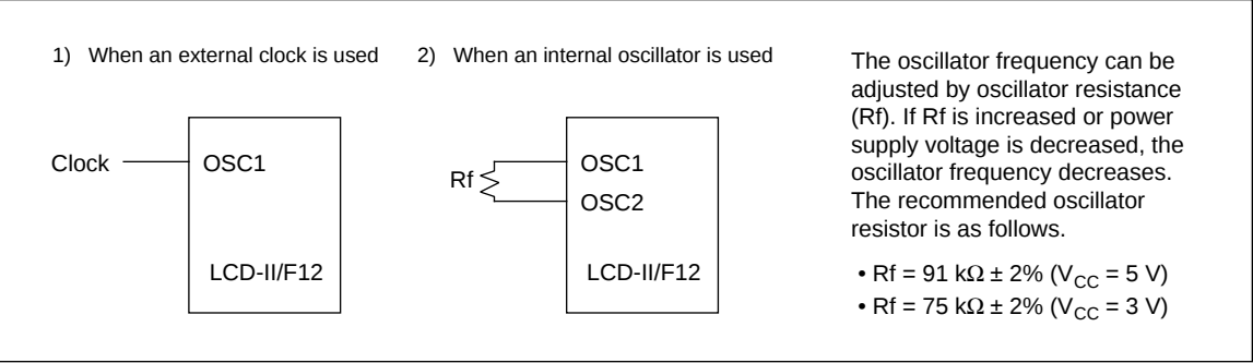
Figure 22 Oscillator Circuit
