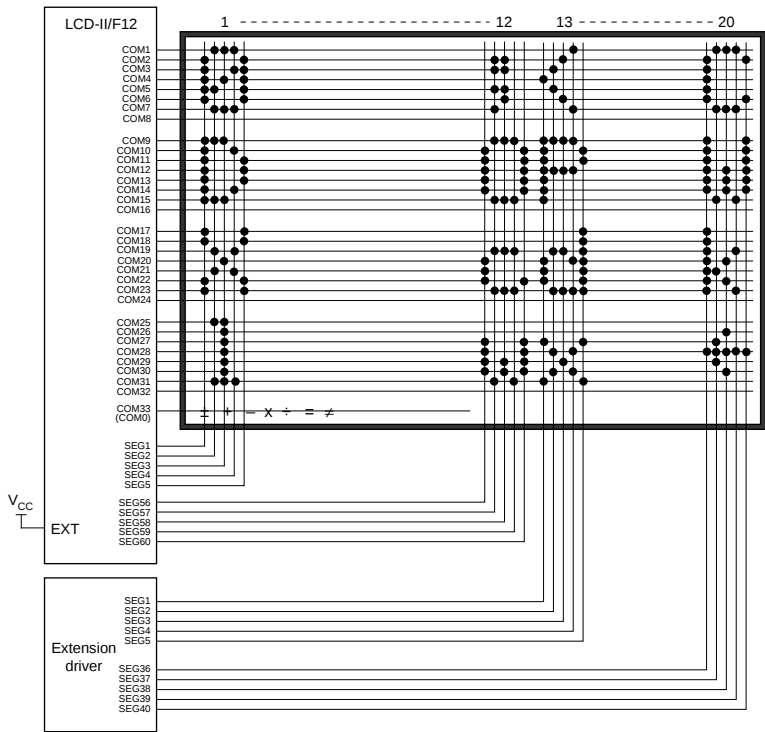
Figure 29 20 × 4-Line + 80 Segment Display (5-Dot Font, 1/33 Duty)
