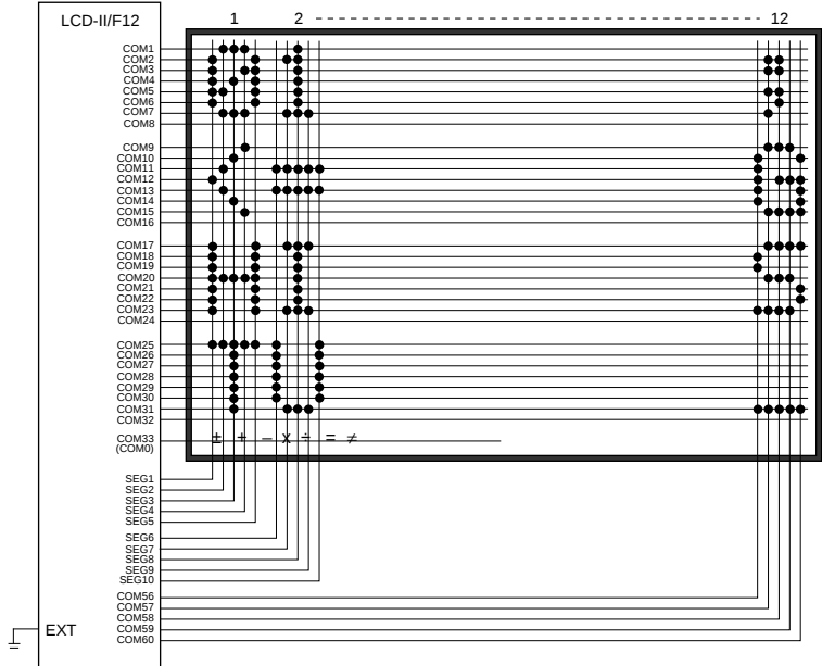
Figure 28 12 × 4-Line + 60 Segment Display (5-Dot Font, 1/33 Duty)
