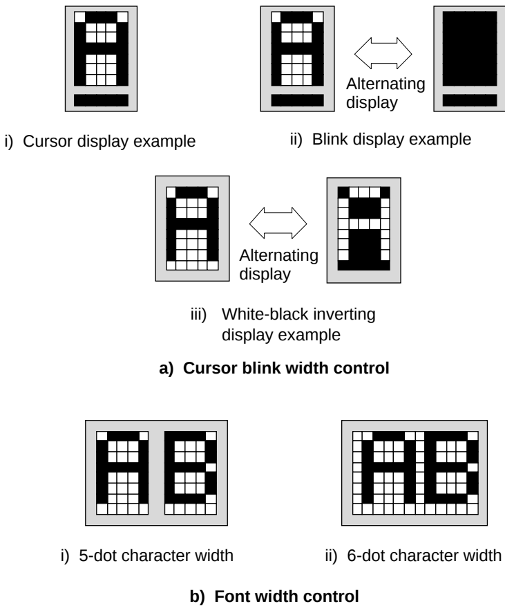
Figure 16 Example of Display Control
