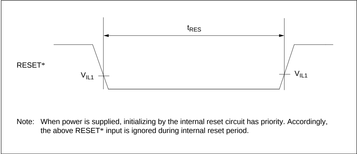
Figure 40 Reset Timing
