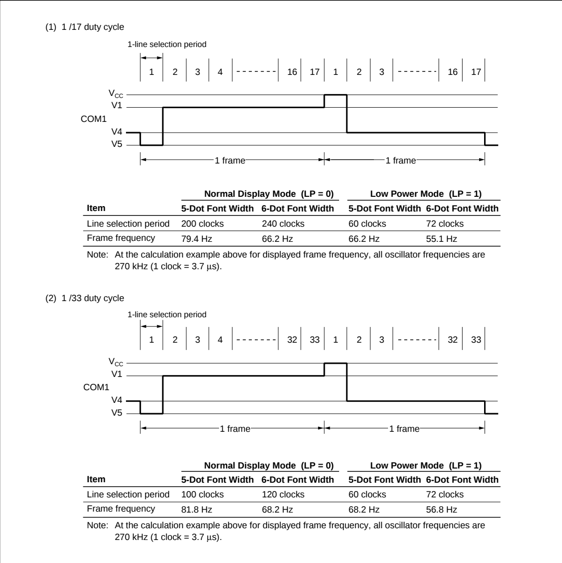
Figure 23 Frame Frequency
