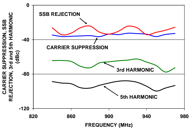
Carrier Suppression, SSB Rejection, 3rd and 5th Harmonic Suppression: V_{CC} = 3.3\text{V} , P_{LO} = +4\text{ dBm}
