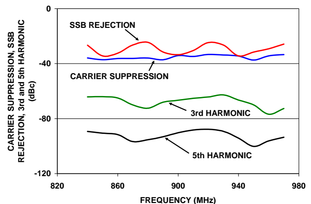
Carrier Suppression, SSB Rejection, 3rd and 5th Harmonic Suppression: V_{CC} = 3.6\text{V} , P_{LO} = +4\text{ dBm}
