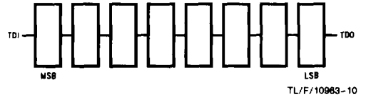
Instruction Register Scan Chain Definition
