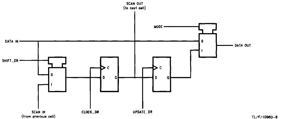
Scan Cell TYPE2
