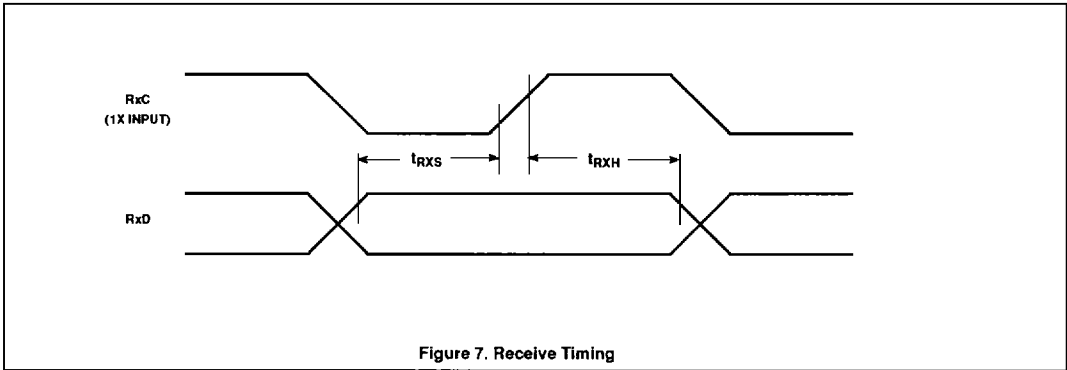
Figure 7. Receive Timing
