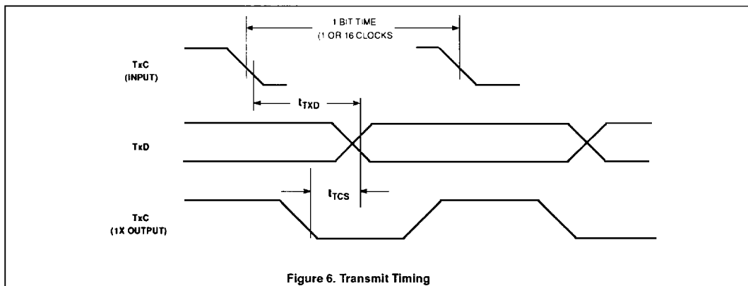
Figure 6. Transmit Timing
