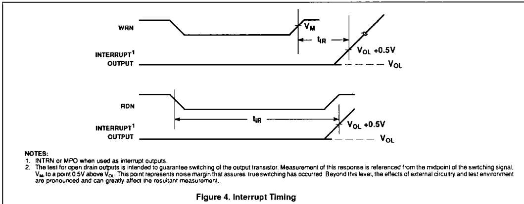
Figure 4. Interrupt Timing
