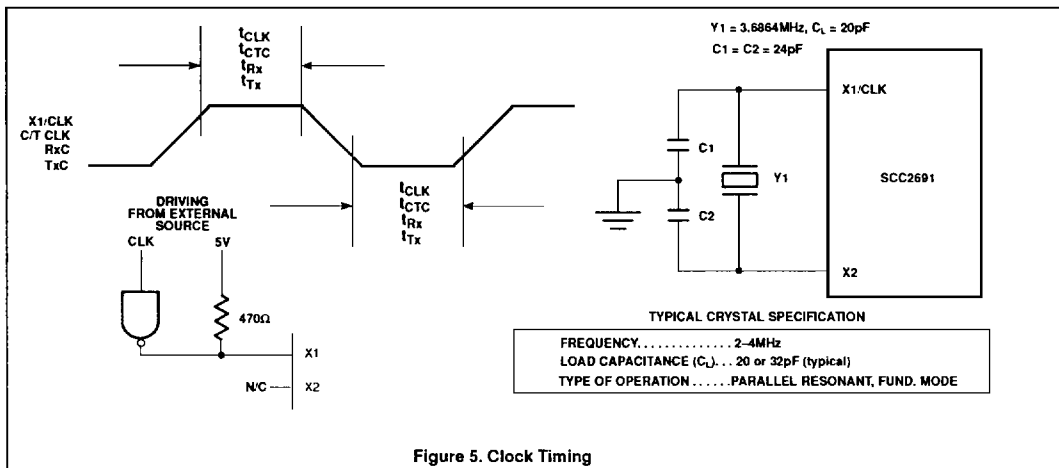
Figure 5. Clock Timing
