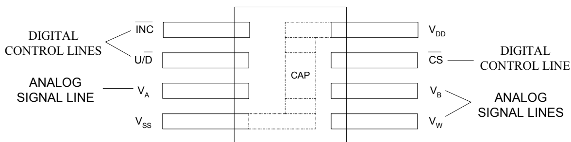
FIGURE 9 – WMS7130/1 LAYOUT
