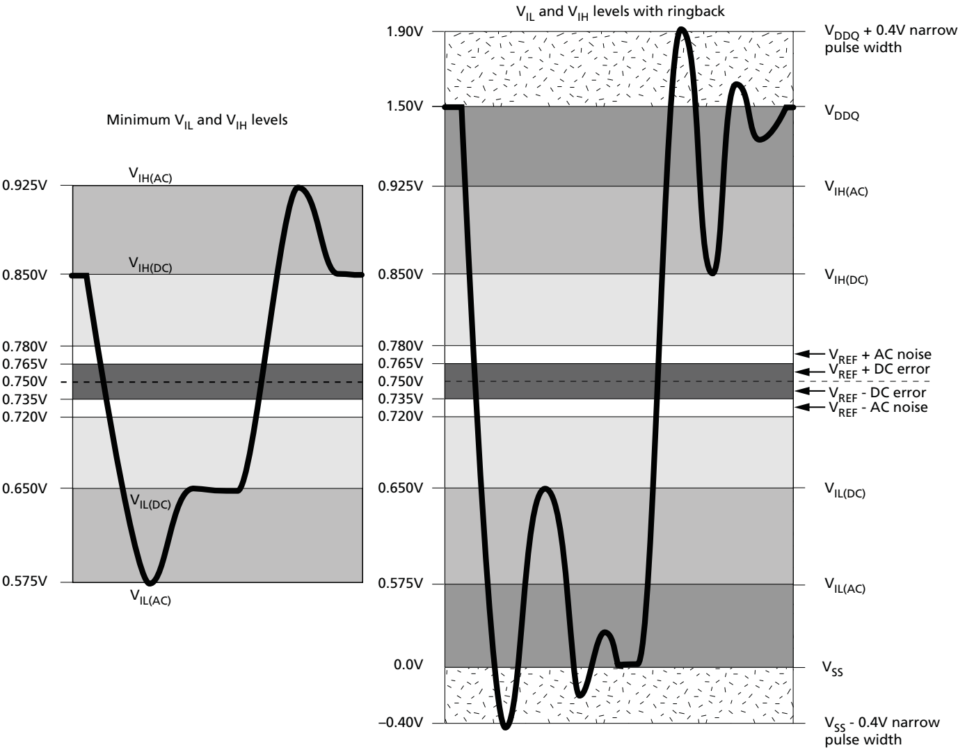
Figure 10: Input Signal
