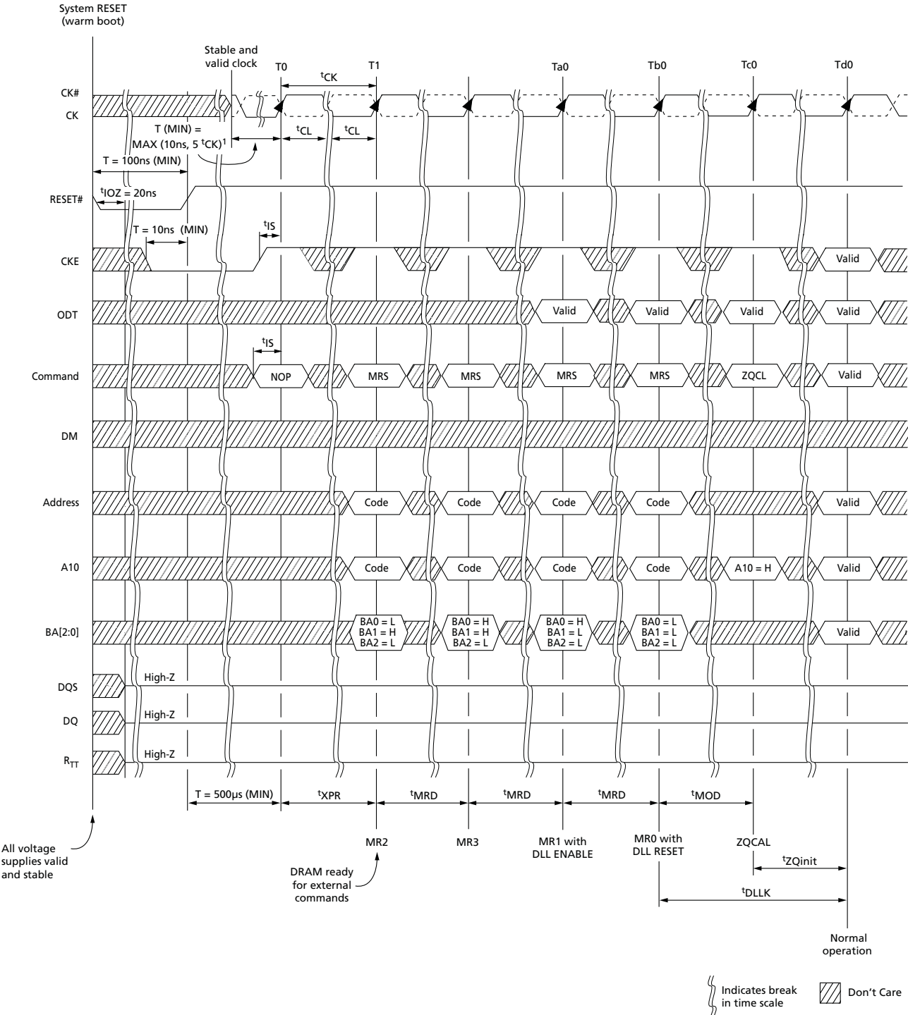
Figure 103: RESET Sequence
