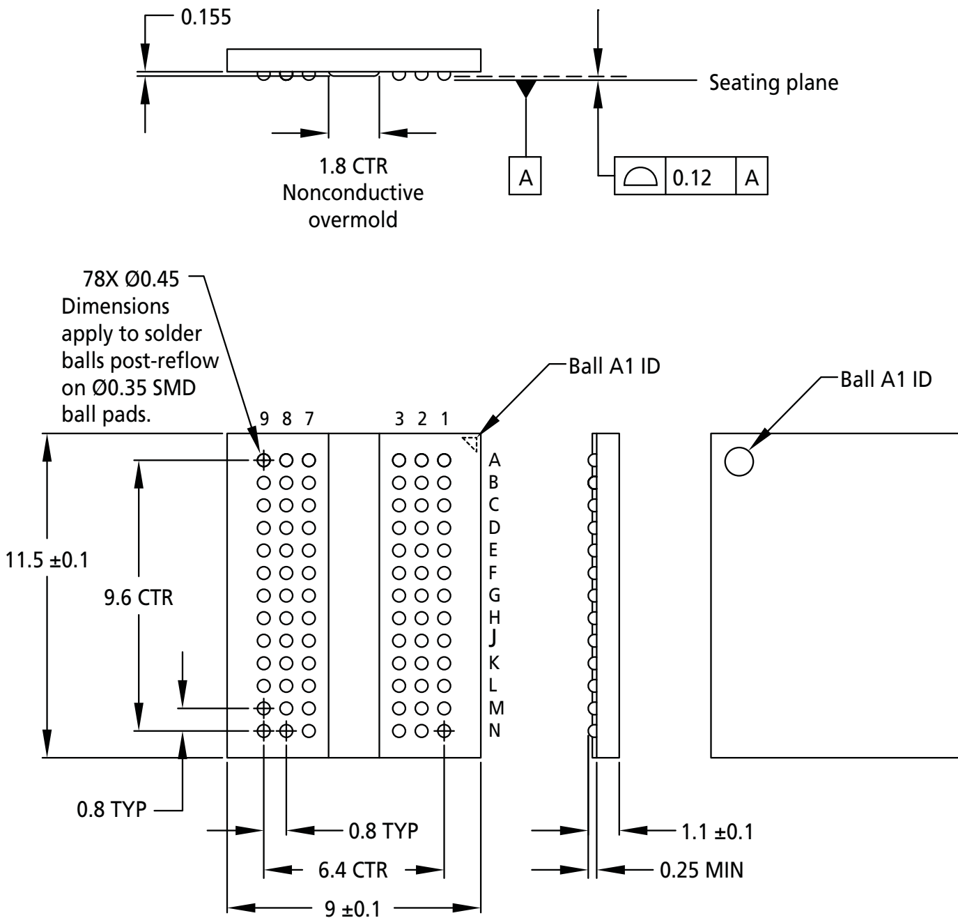
Figure 6: 78-Ball FBGA – x4, x8 (HX)
