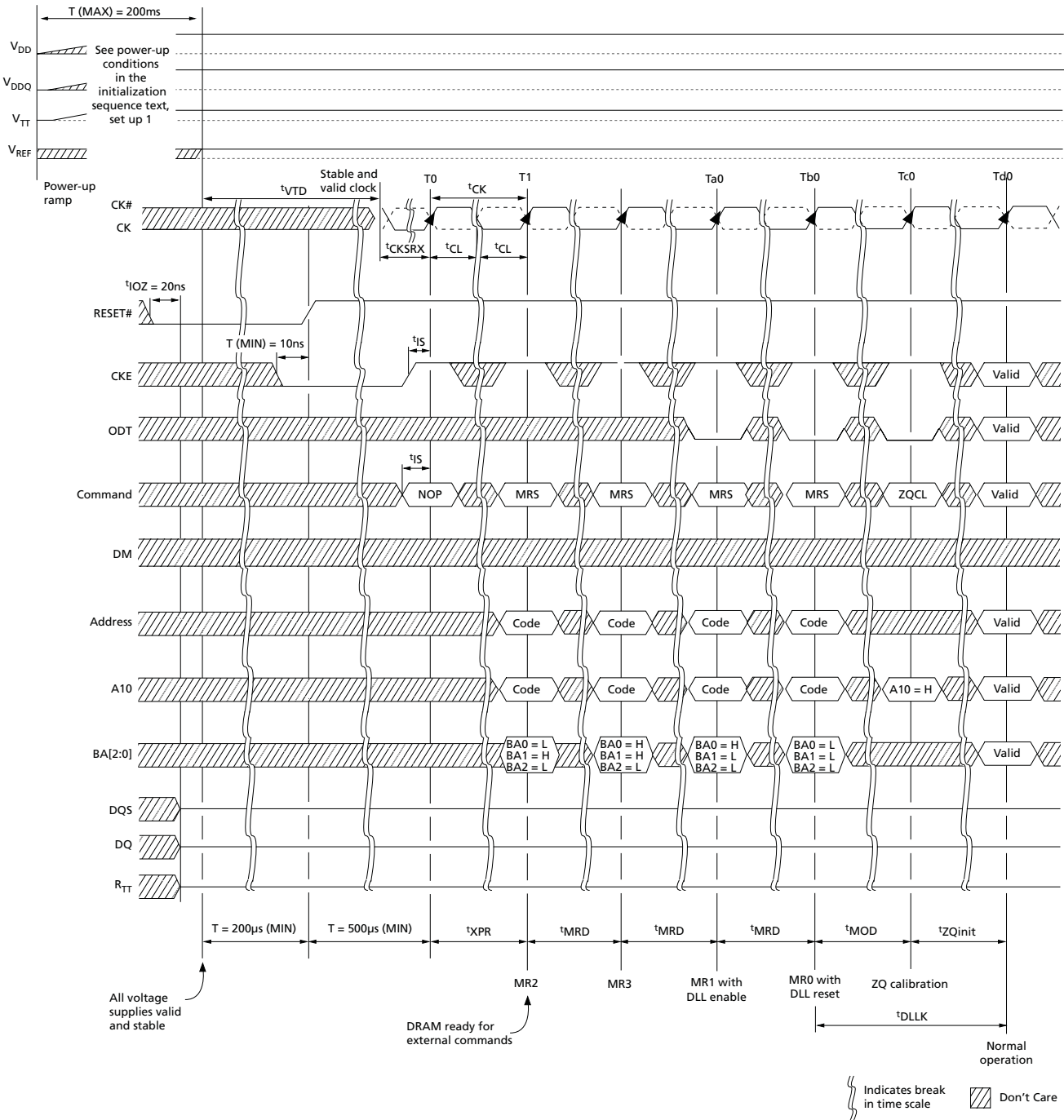
Figure 45: Initialization Sequence
