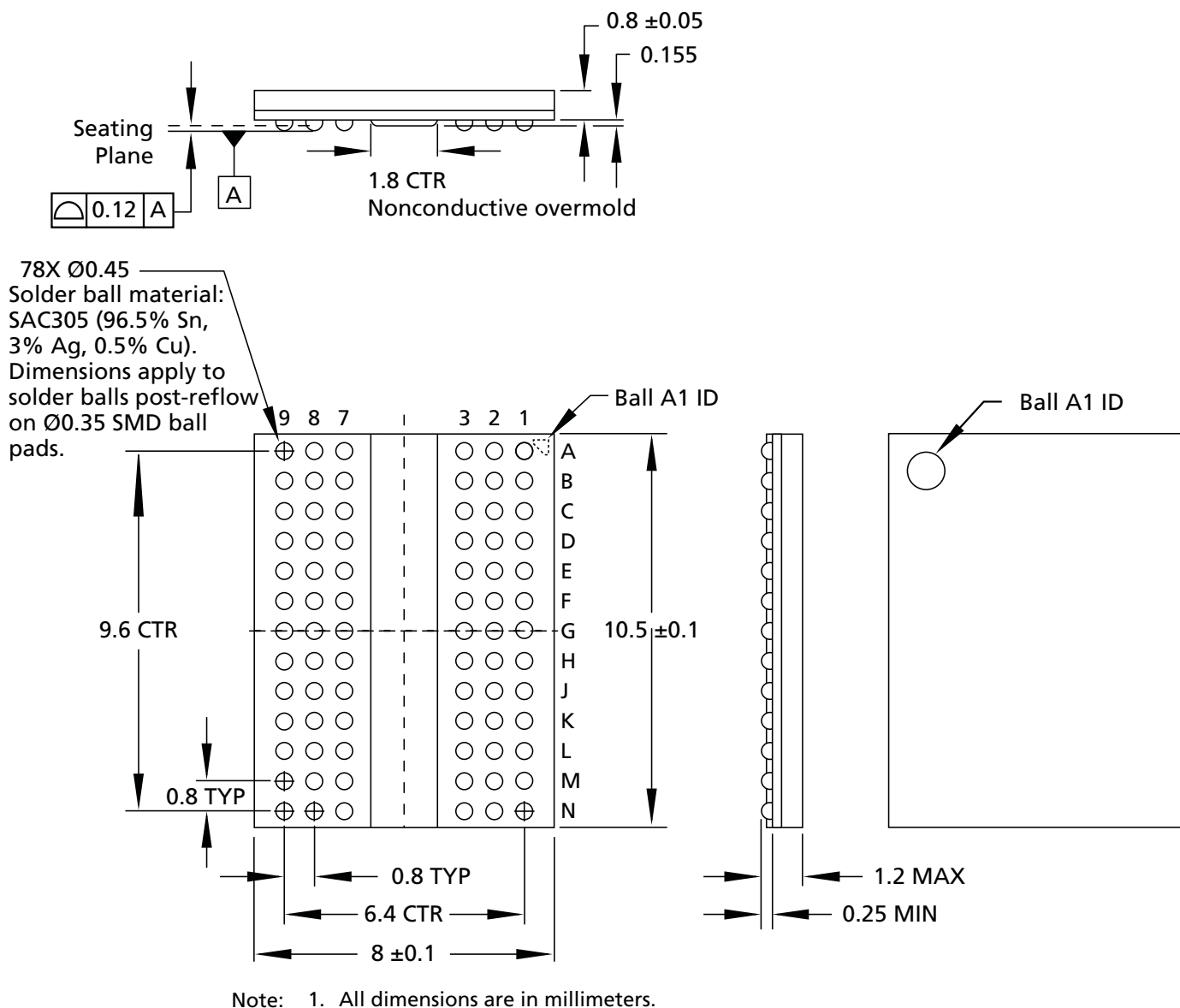
Figure 5: 78-Ball FBGA – x4, x8 (DA)
