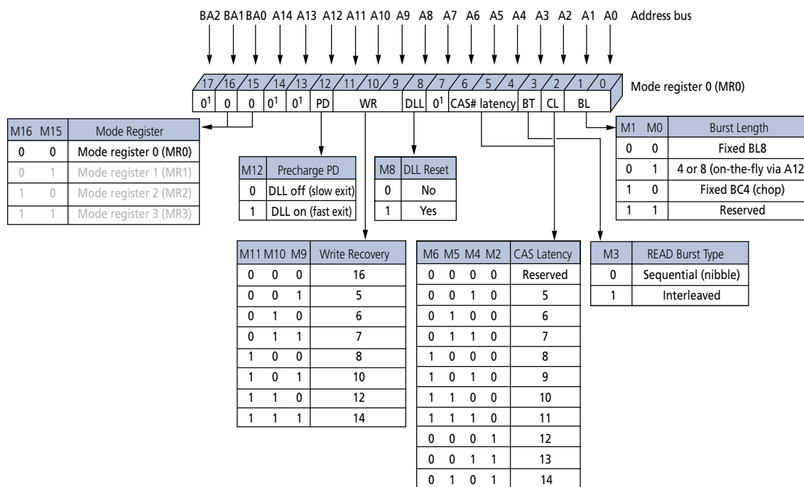
Figure 48: Mode Register 0 (MR0) Definitions
