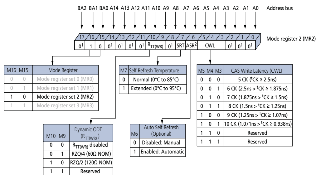
Figure 52: Mode Register 2 (MR2) Definition
