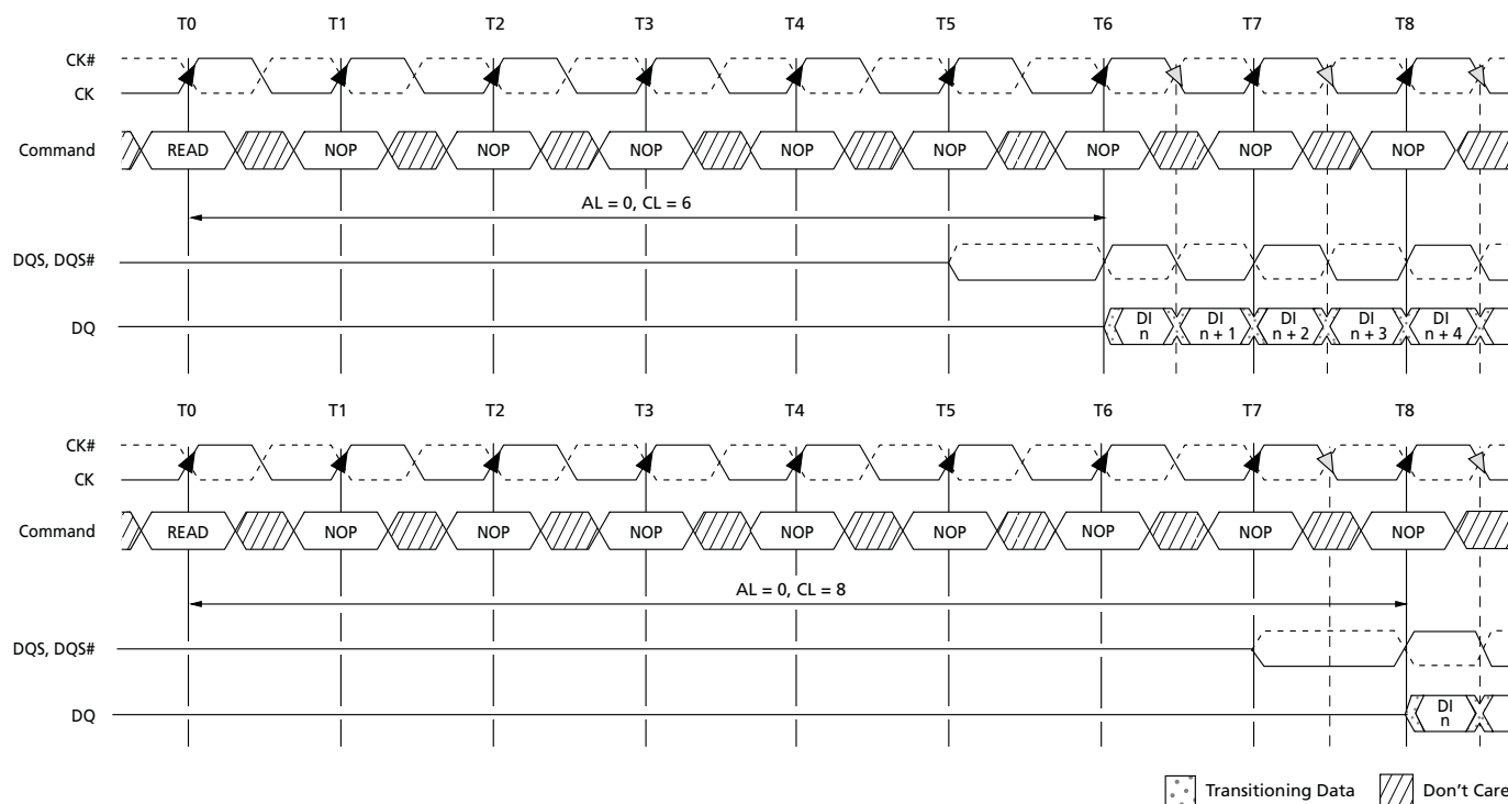
Figure 49: READ Latency
