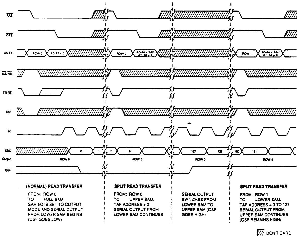
Figure 5 TYPICAL SPLIT READ TRANSFER INITIATION SEQUENCE
