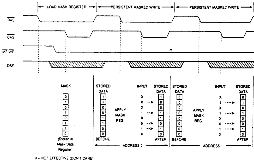
Figure 3 PERSISTENT MASKED WRITE EXAMPLE
