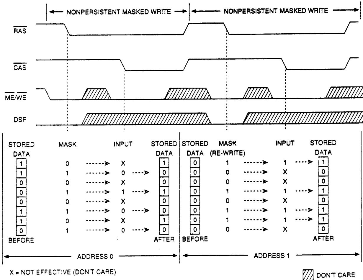
Figure 2 NONPERSISTENT MASKED WRITE EXAMPLE
