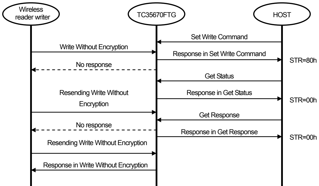
Figure 4-25 command processing sequence of wired interface
