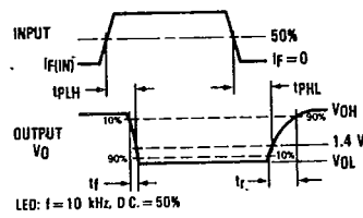
Switching Test Curve for Inverters
