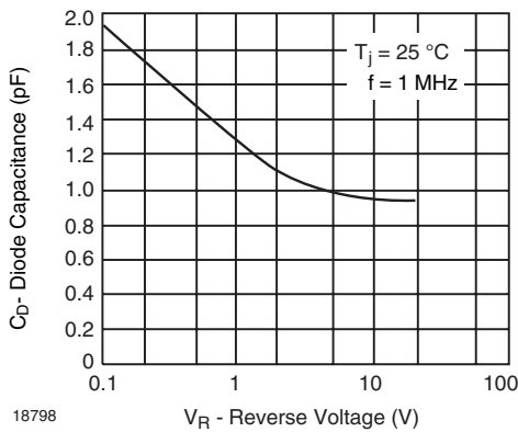
Figure 1. Diode Capacitance
