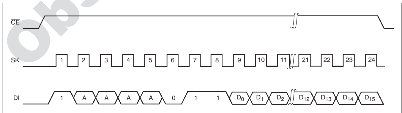
Figure 2. RAM Write
