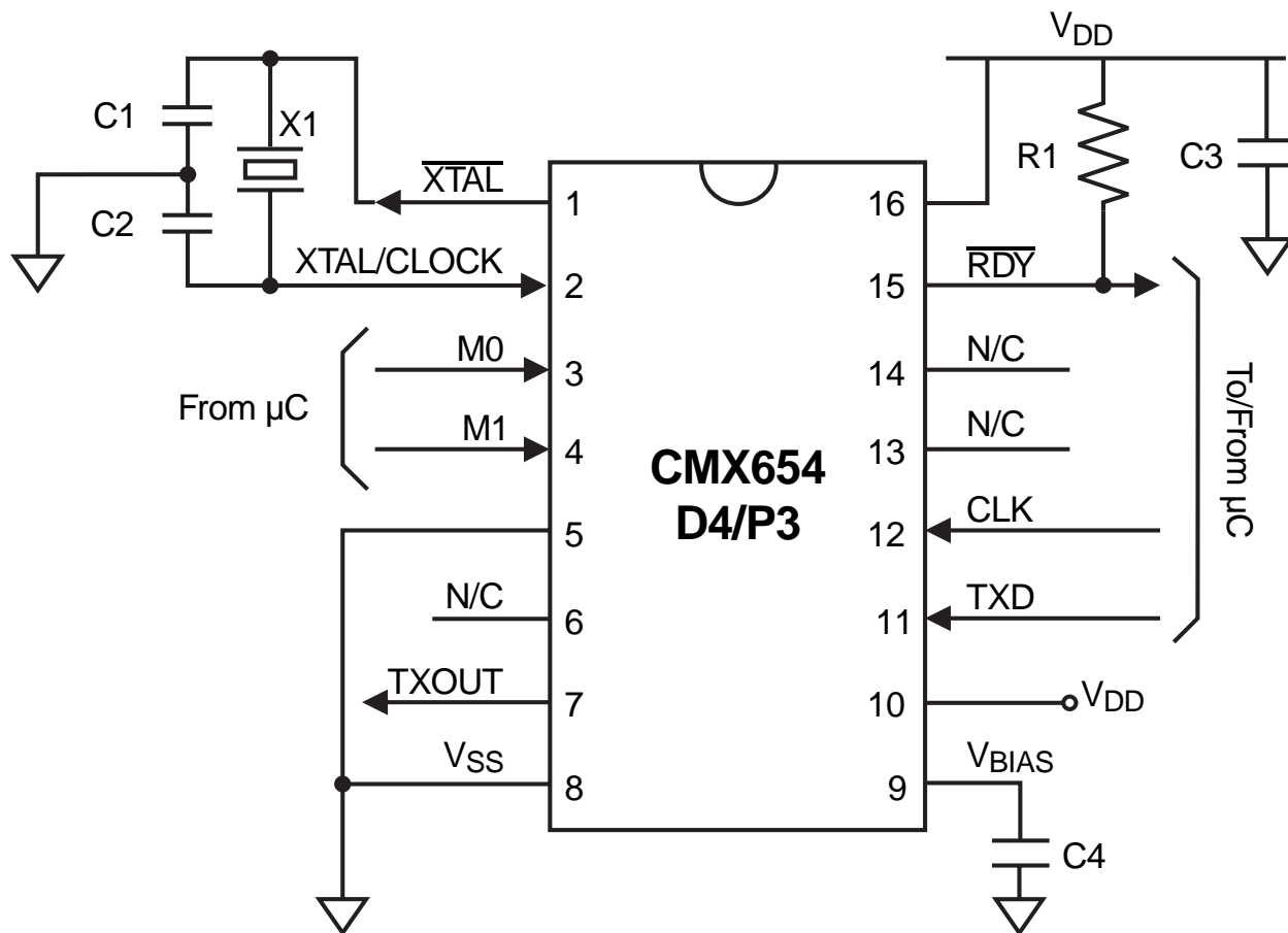
Figure 2: External Components
