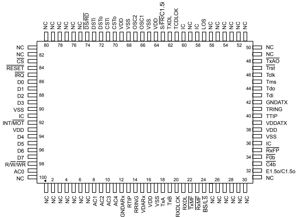
Figure 2 - Pin Connections
