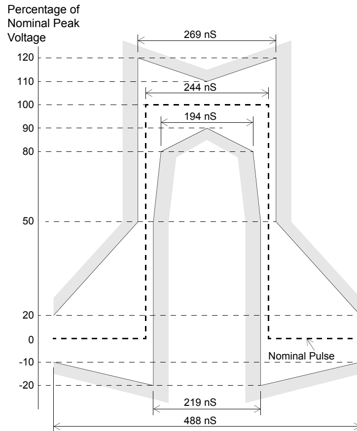
Figure 8 - Pulse Template (G.703)(E1)
