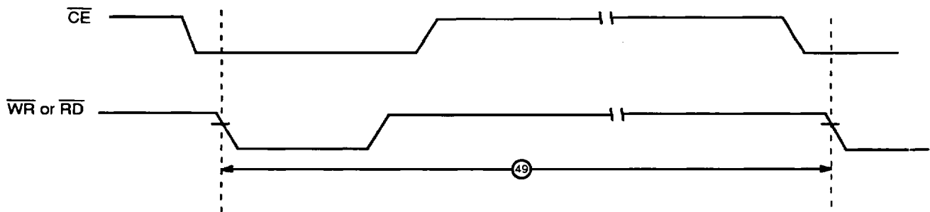
Figure 17. Cycle Timing
