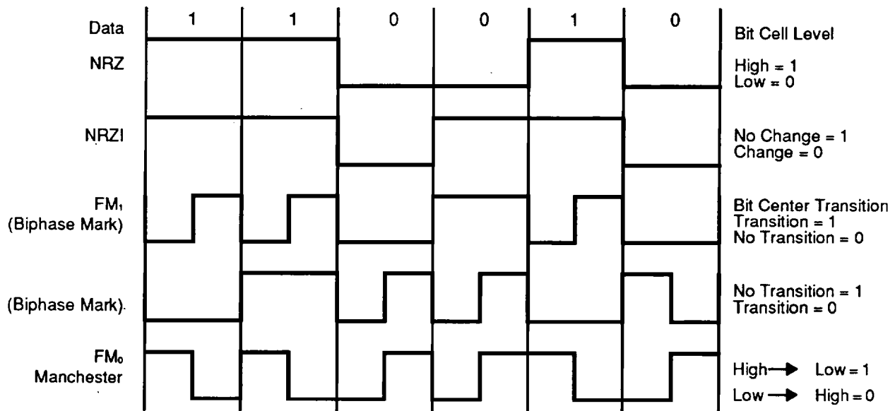
Figure 5. Data Encoding Methods
