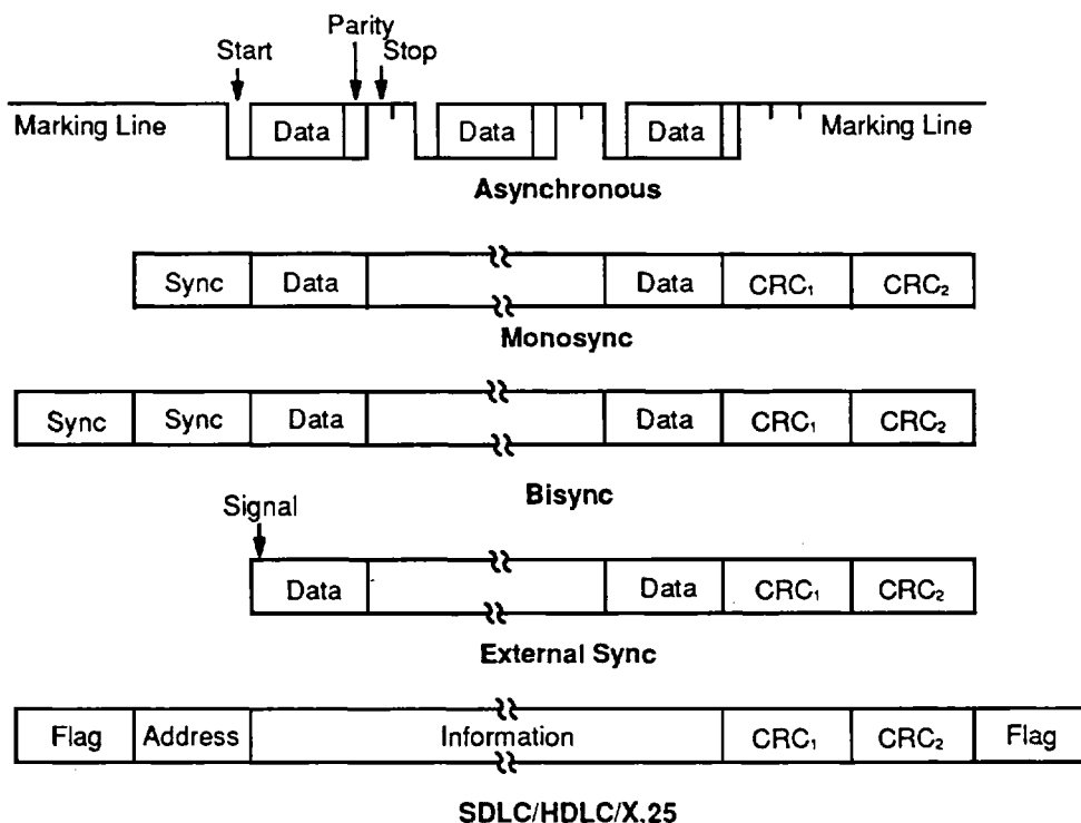
Figure 2. SCC Protocols
