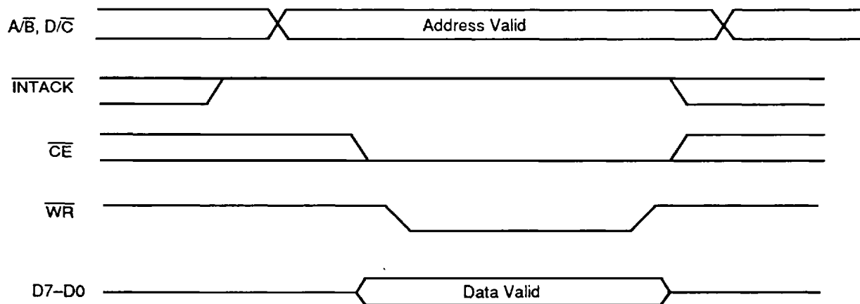
Figure 9. Read Cycle Timing
