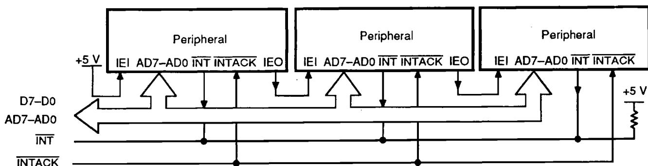
Figure 6. Z-Bus Interrupt Schedule
