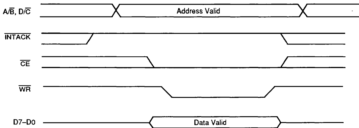
Figure 10. Write Cycle Timing
