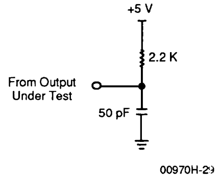
Open-Drain Test Load
