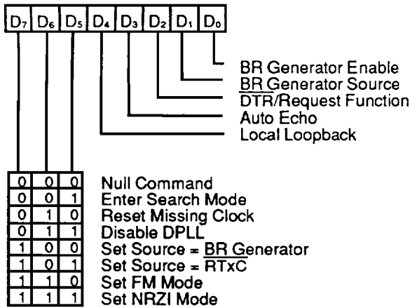
Figure 8. Write Register Bit Functions (continued)
