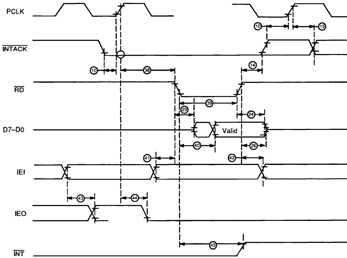
Figure 15. Interrupt Acknowledge Timing
