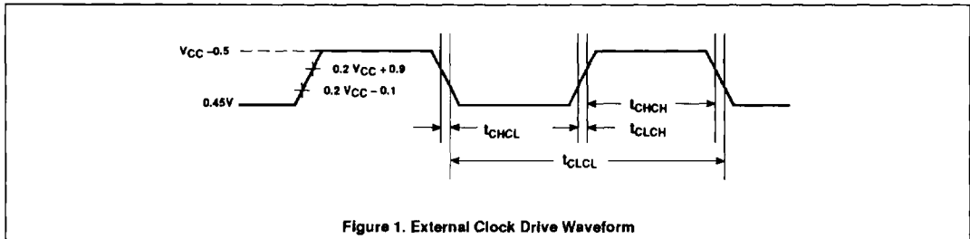
Figure 1. External Clock Drive Waveform
