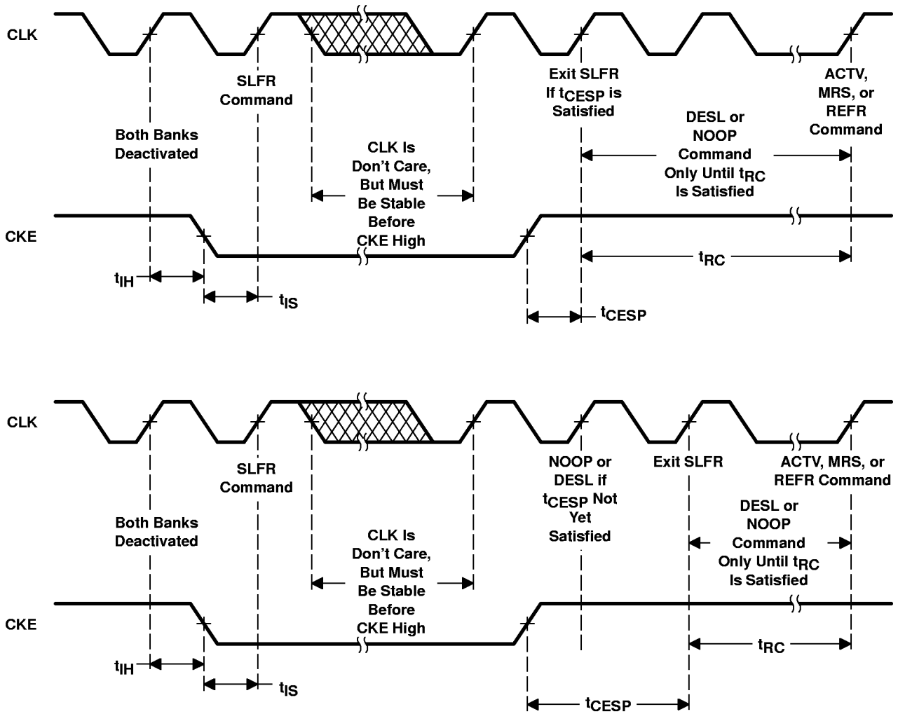
Figure 19. Self-Refresh Operation
