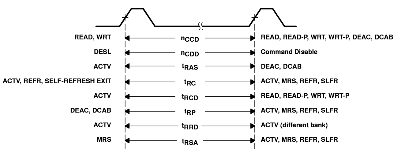
Figure 11. Command-to-Command Parameters
