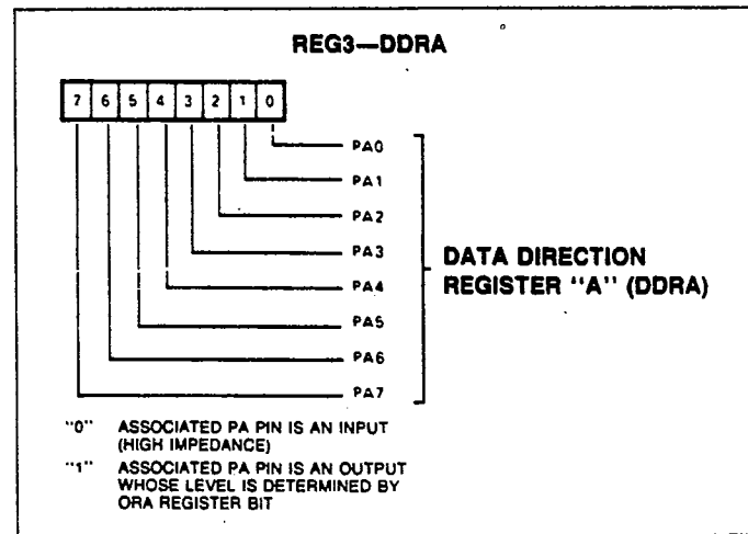
Figure 8. Data Direction Register A (DDRA)
