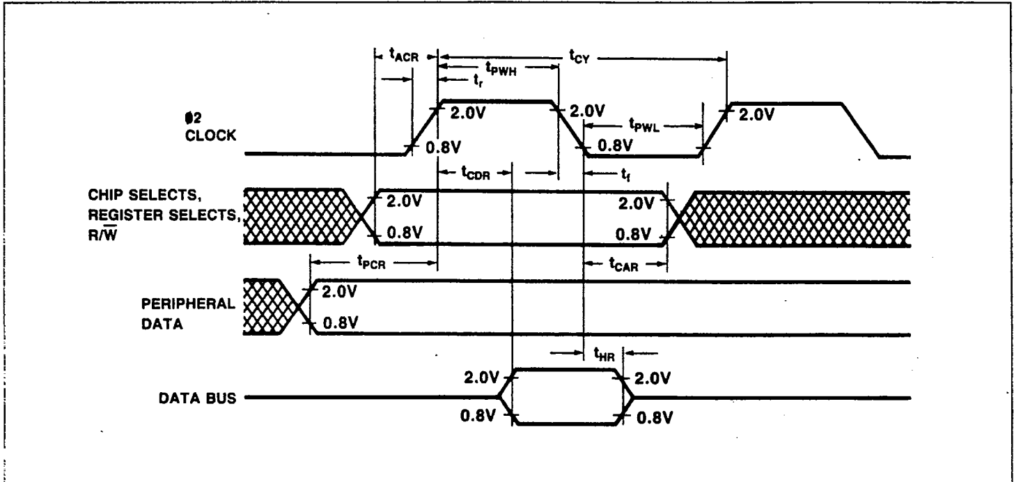
Figure 32a. Read Timing Waveforms
