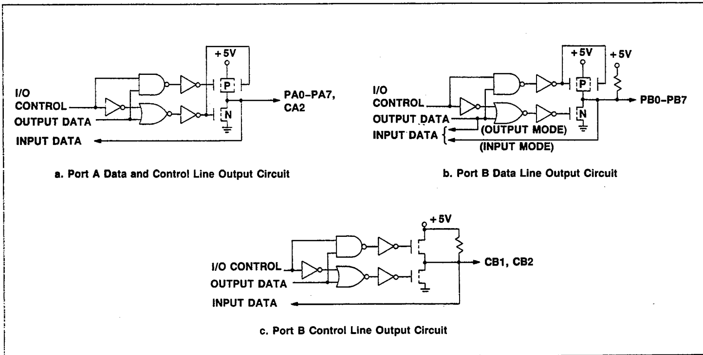
Figure 3. Port A and B Output Circuits
