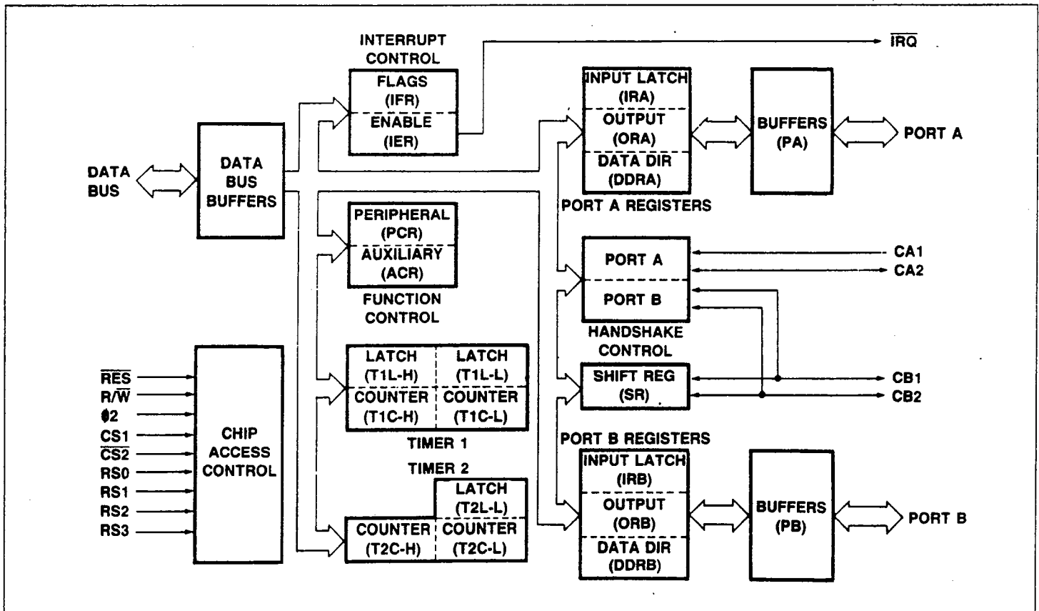
Figure 4. R65NC22 VIA Block Diagram
