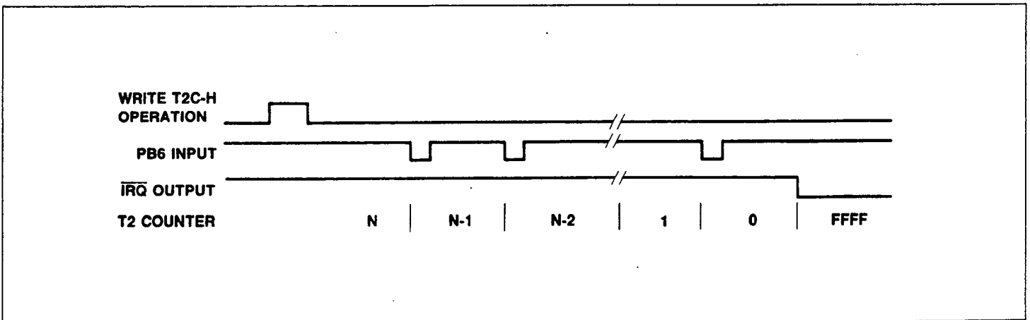
Figure 19. Timer 2 Pulse Counting Mode
