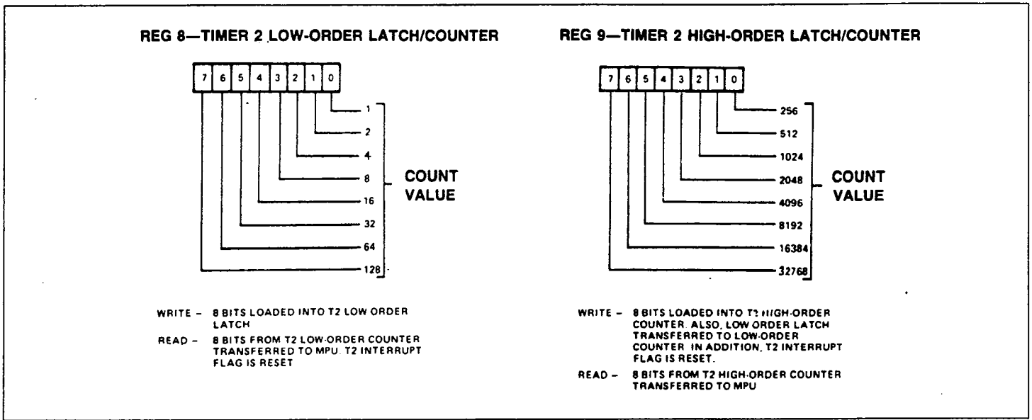
Figure 17. Timer 2 (T2) Latch/Counter Registers
