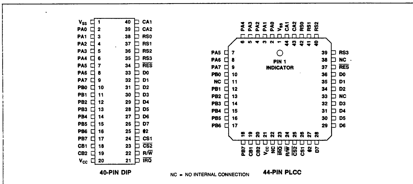
Figure 1. R65NC22 Pin Assignments
