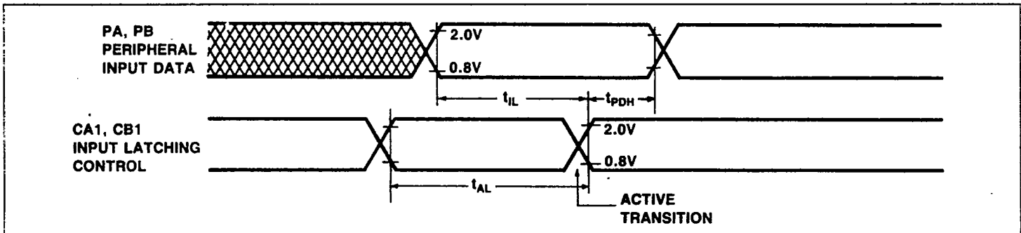
Figure 31e. Peripheral Data Input Latching Timing
