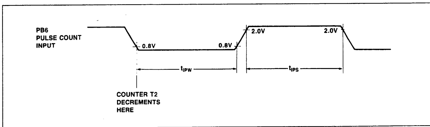
Figure 31i. Pulse Count Input Timing
