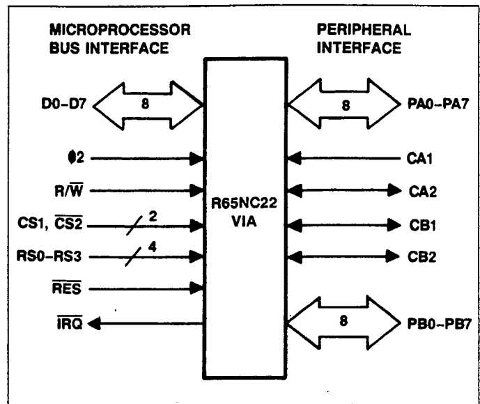
Figure 2. R65NC22 VIA Interface Signals
