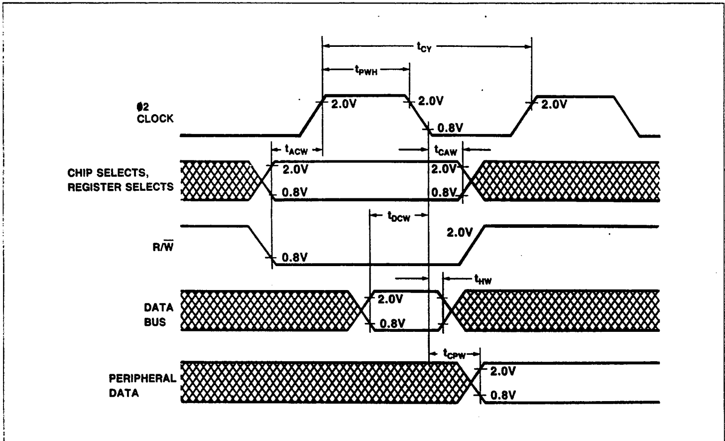
Figure 32b. Write Timing Waveforms
