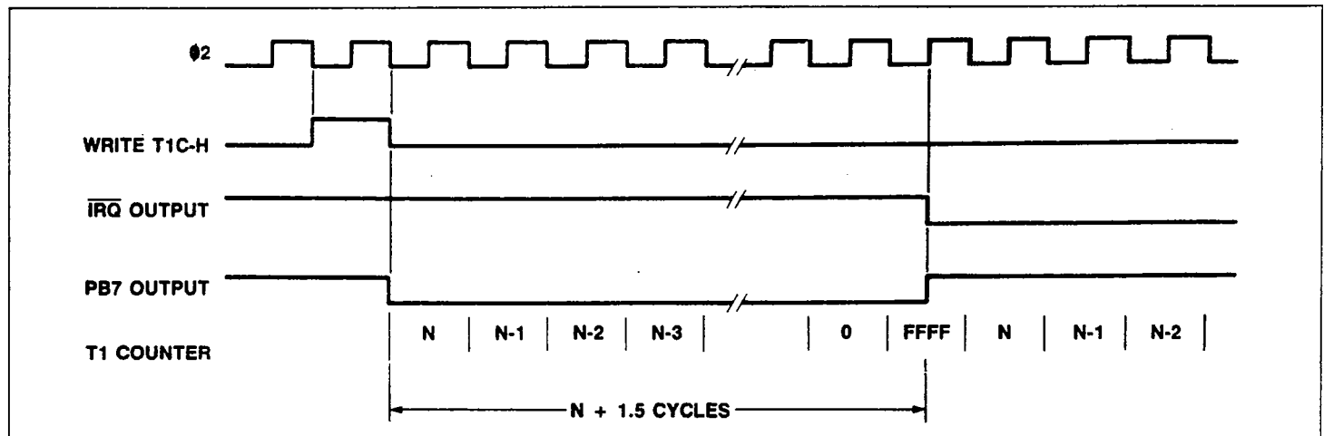
Figure 15. Timer 1 One-Shot Mode Timing
