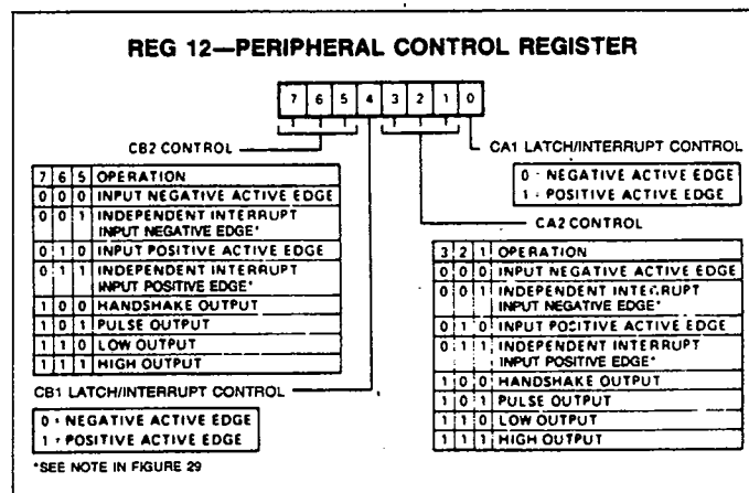
Figure 11. Peripheral Control Register (PCR)
