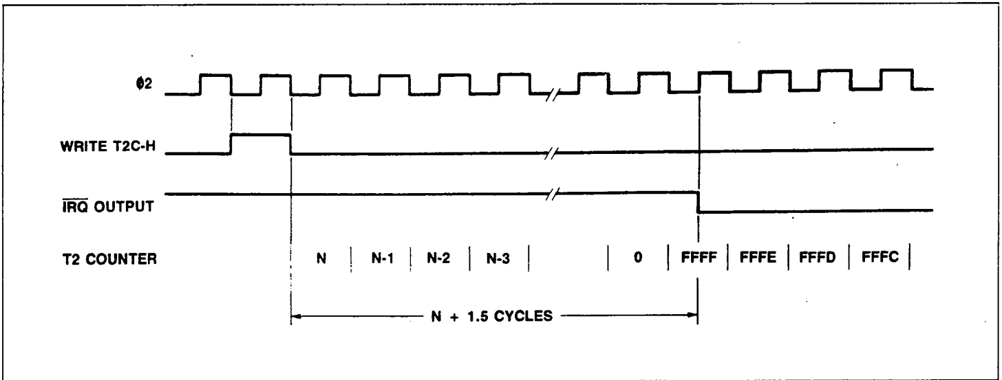
Figure 18. Timer 2 One-Shot Mode Timing
