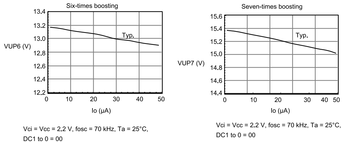
Figure 63 Booster (cont)
