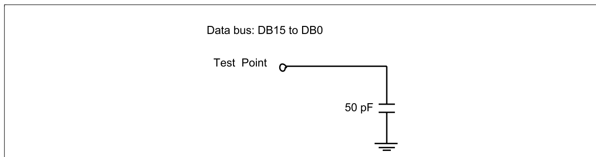
Figure 64 Load Circuit
