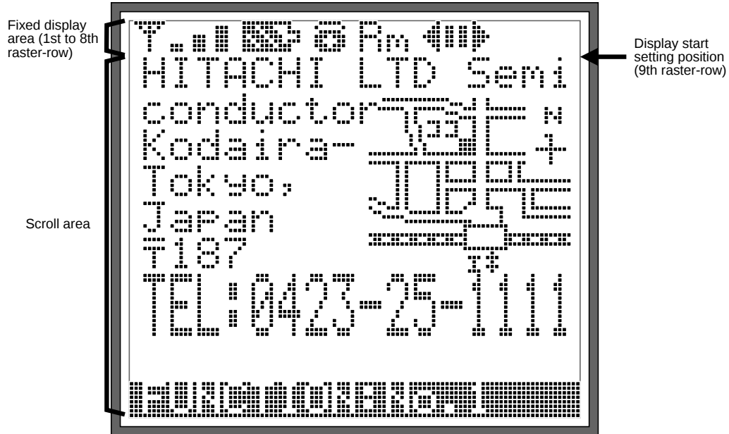
Figure 51 Example of the initial screen in the partial smooth scroll mode
