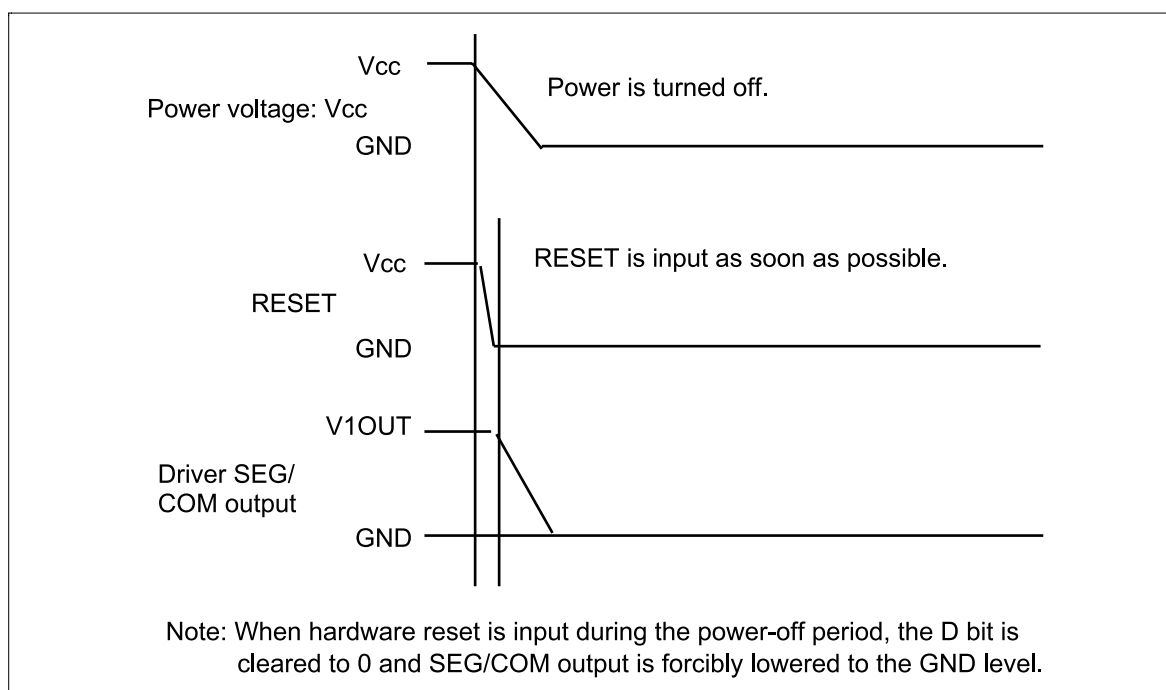
Figure 73 Power-off Timing
