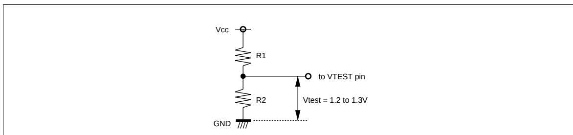
Figure 38 Circuit to for Generating VTEST Pin Voltage
