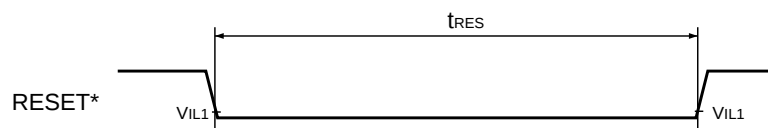
Figure 69 Reset Timing
