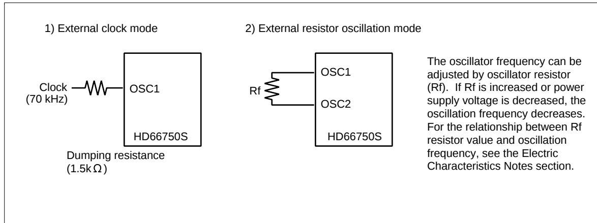
Figure 32 Oscillation Circuits
