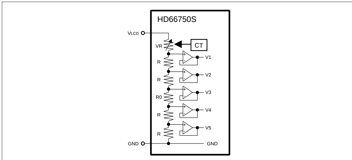
Figure 43 Contrast Adjuster
