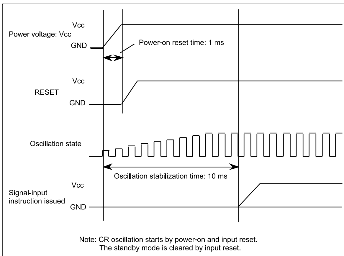
Figure 71 Power-on Timing
