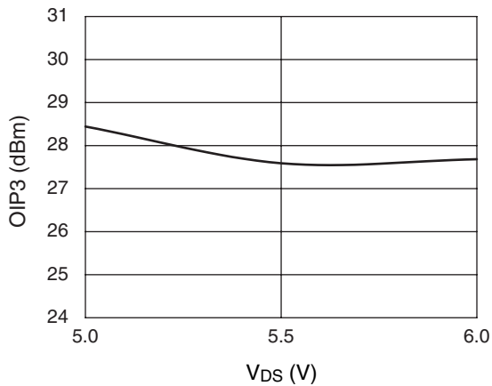
Two-Tone Output Third-Order Intercept @ 39 GHz
