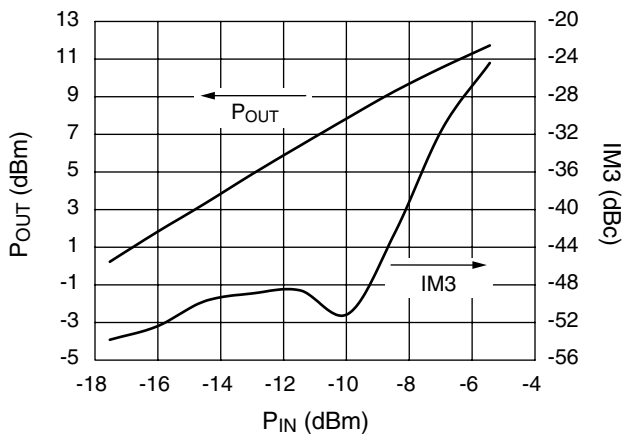
Output Power and Relative Third-Order Intermodulation Products F = 39 GHz, V DS = 5.5 V
