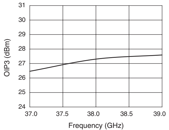
Two-Tone Output Third-Order Intercept @ V DS = 5.5 V
