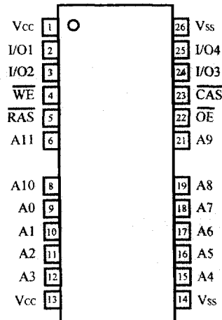
24(26) TSOP II
