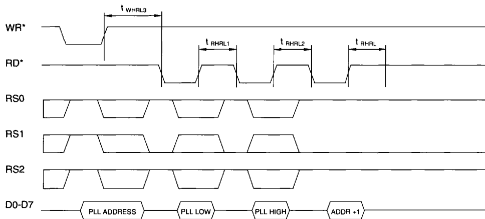
Read Two bytes PLL Register then PLL Address Register
