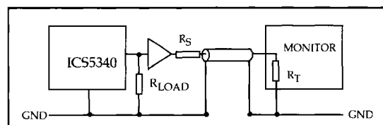
Figure 2 - Buffered Signal
