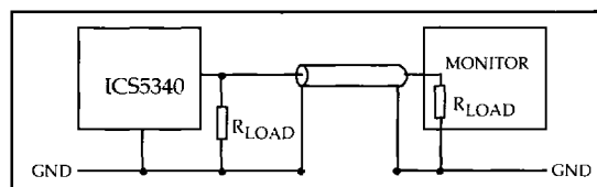
Figure 1 - Double Termination
