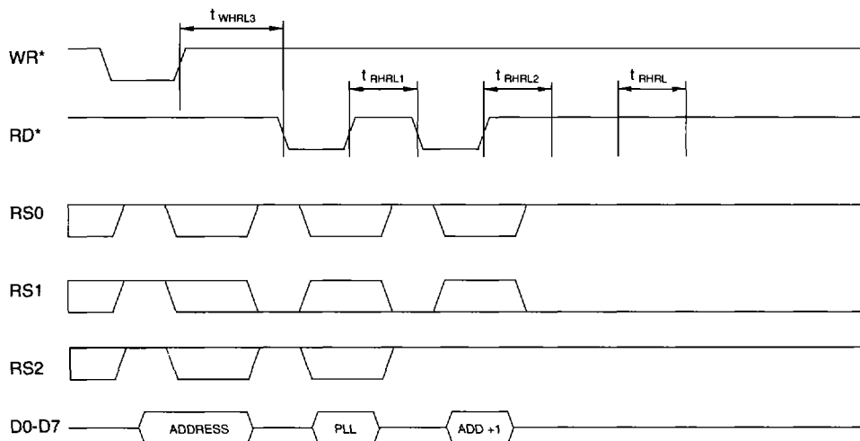
Read One Byte PLL Register then PLL Address Register
