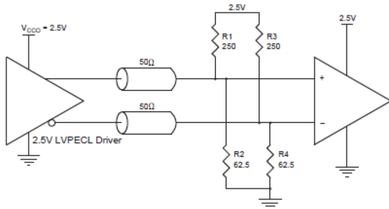
Figure 8. 2.5V LVPECL Driver Termination Example
