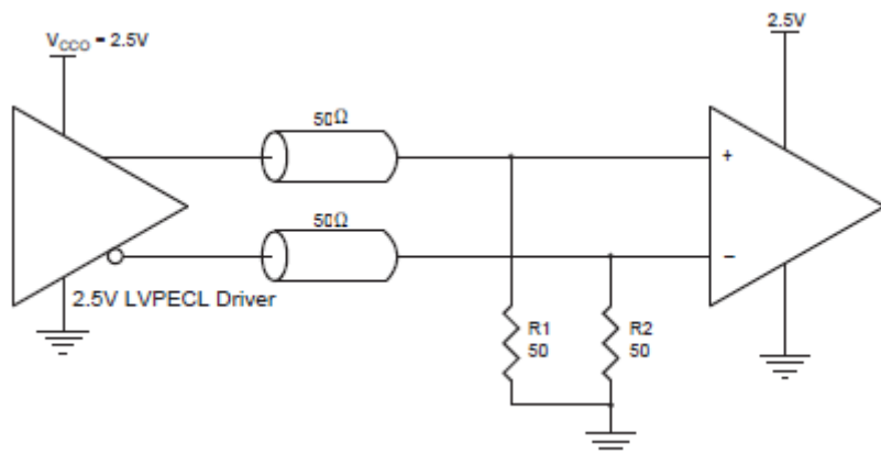
Figure 9. 2.5V LVPECL Driver Termination Example
