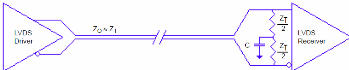
Figure 12. Optional LVDS Termination
