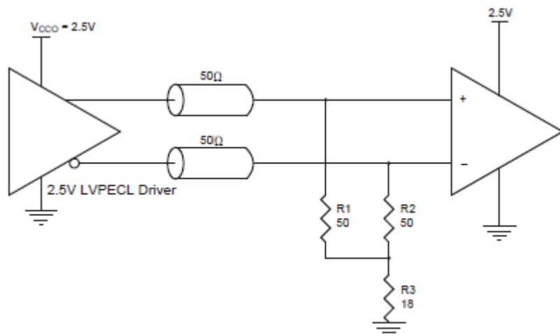
Figure 10. 2.5V LVPECL Driver Termination Example
