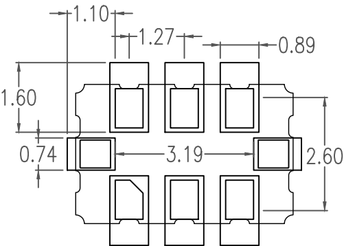
RECOMMENDED LAND PATTERN DIMENSIONS
