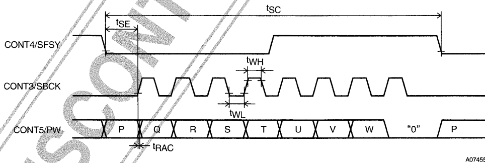
Figure 3 Subcode Output
