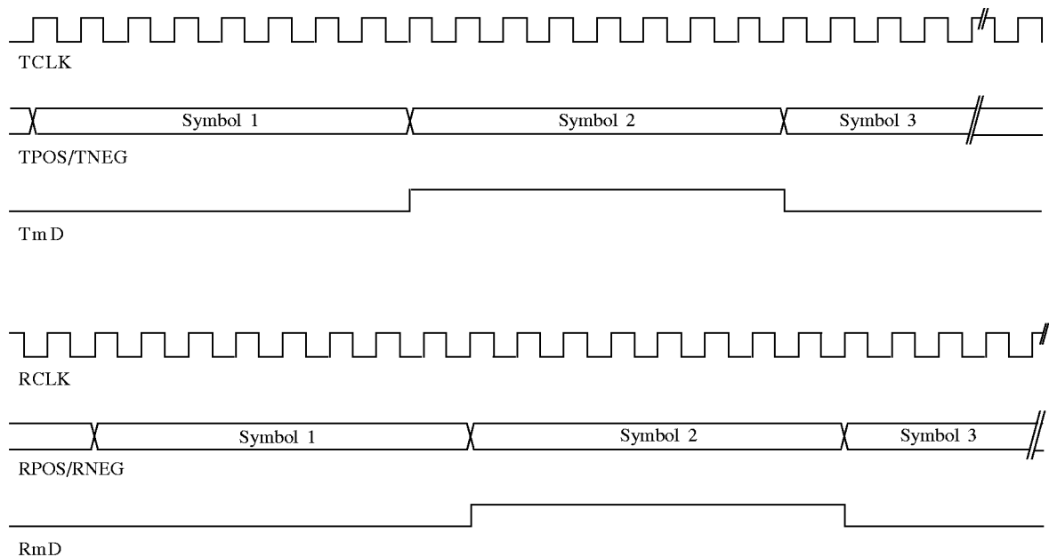
Figure 2. Use of support signals to identify symbols in E1/E2 frame
