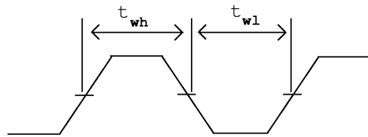
TmCLK and RmCLK clock pulse widths
