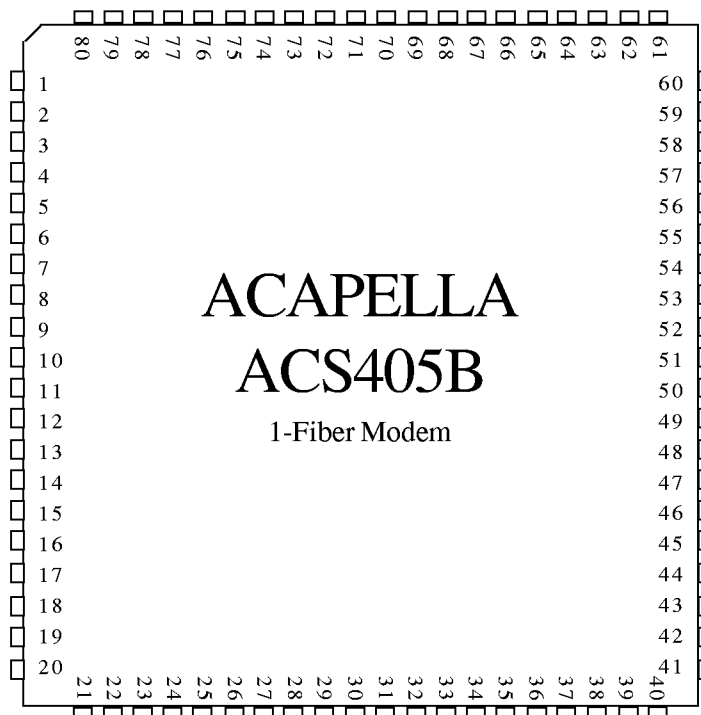
Figure 7. Top view of 80 pin TQFP package
