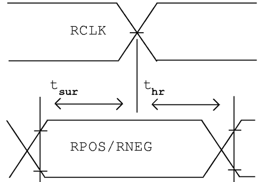
Receive set-up and hold times
