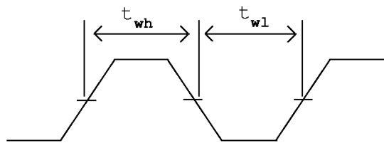
TCLK and RCLK clock pulse widths
