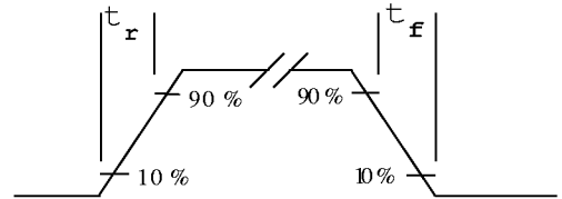
Digital outputs rise and fall times
