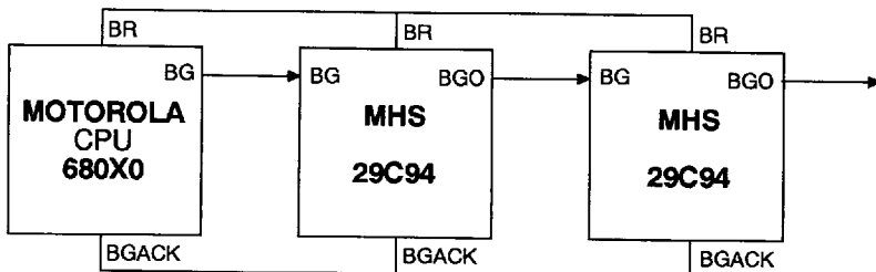
Figure 12b. MOTOROLA Daisy Chain
