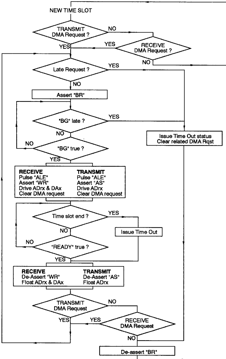
Figure 10. DMA cycle with INTEL host CPU.
