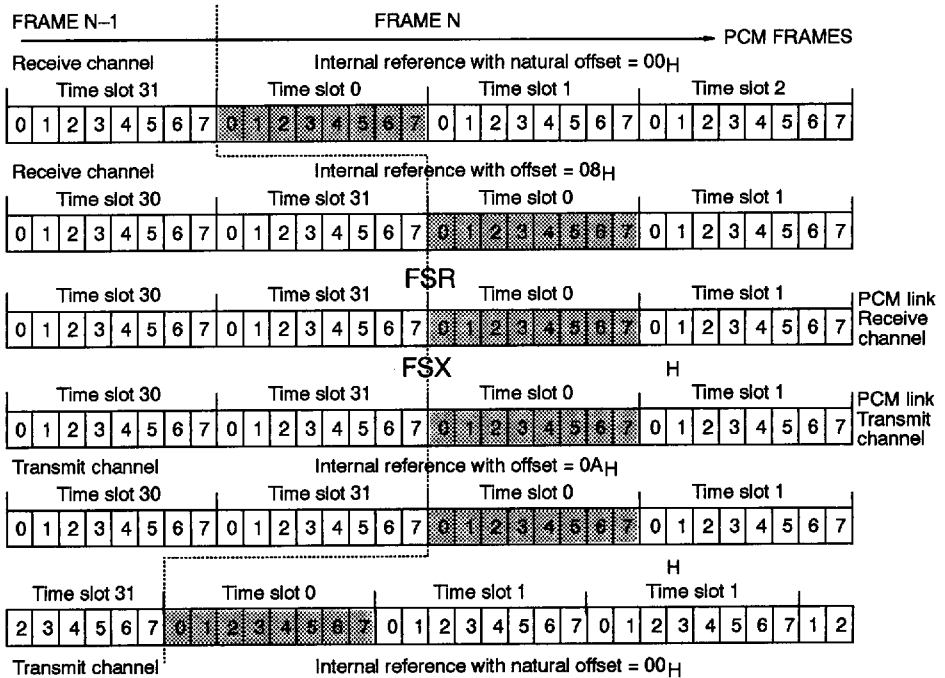
Figure 5. Internal References and Offsets.
