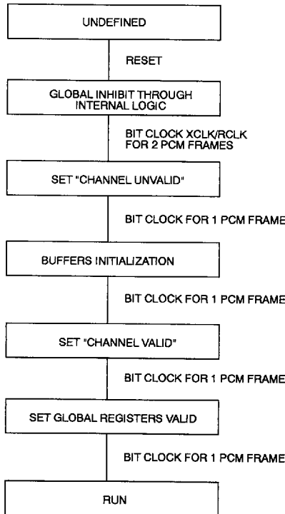
Figure 14. Example of initialization procedure.
