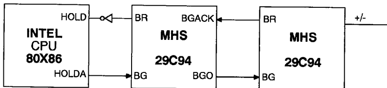
Figure 12a. INTEL Daisy Chain
