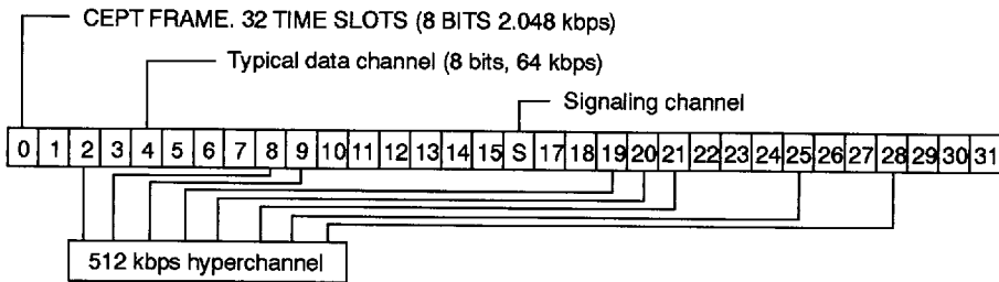
Figure 8. 512 kbps hyperchannel
