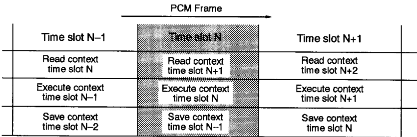
Figure 4. Context Monitor pipe-line.
