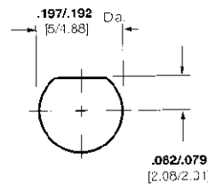
Maximum Panel Thickness .093 [2.36] Recommended Panel Cutout
