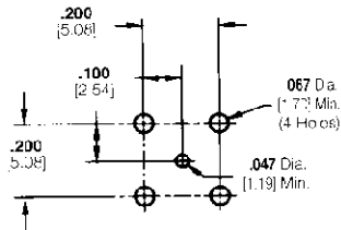
Recommended PC Board Layouts
