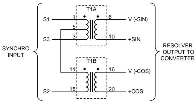
FIGURE 16A. 400 HZ SYNCHRO AND RESOLVER TRANSFORMER MECHANICAL OUTLINES AND ELECTRICAL SCHEMATICS
