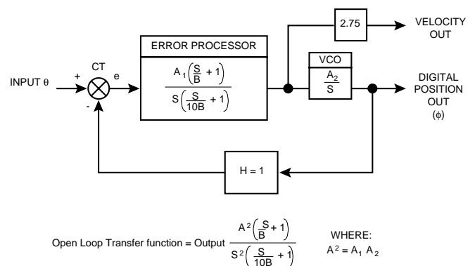
FIGURE 6. CONTROL LOOP BLOCK DIAGRAM
