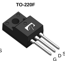
AOTF380A60CL
