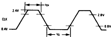
External Clock Input (24 MHz Max)
