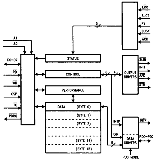
Block Diagram of the Parallel Port Logic
