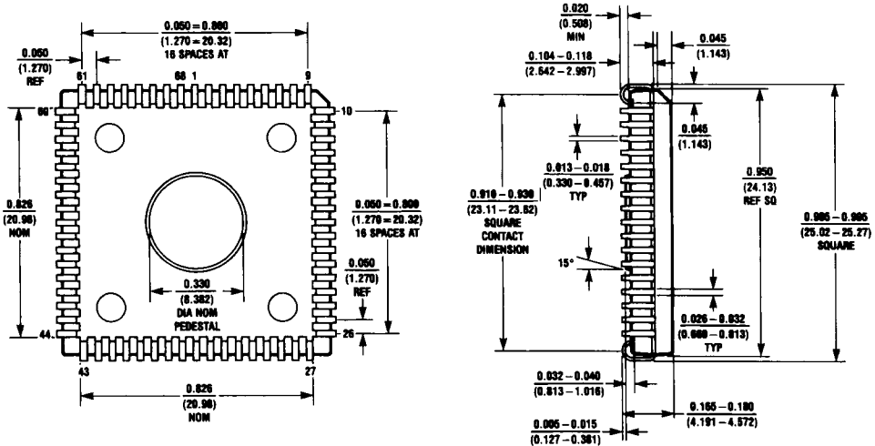
68-Lead Plastic Chip Carrier (V) Order Number PC16553V NS Package Number V68A
