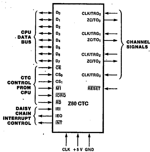
Figure 1. Pin Functions
