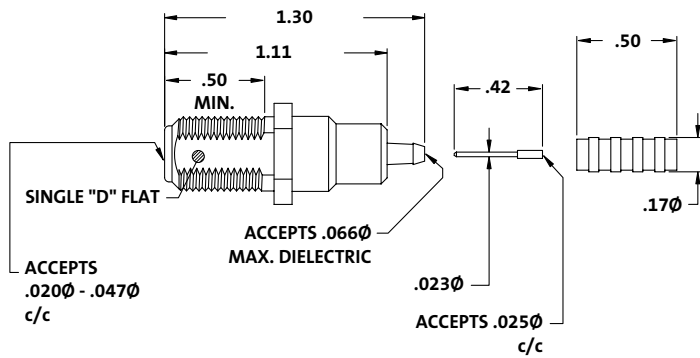
RG-179B/U Double Braided Female Coax Connector
