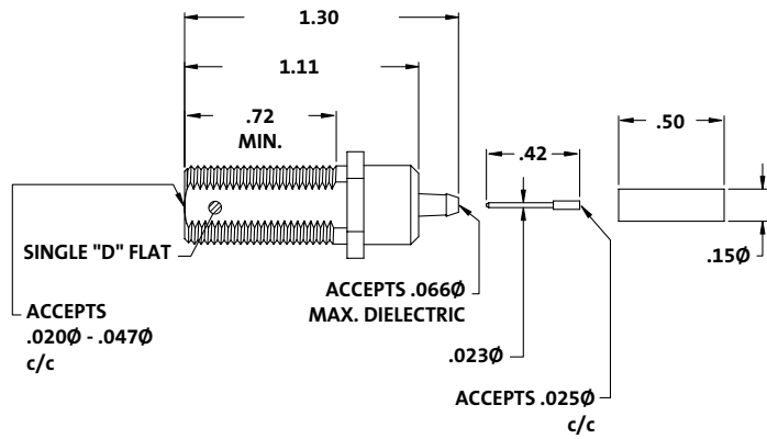
RG-179B/U Long Thread Female Coax Connector
