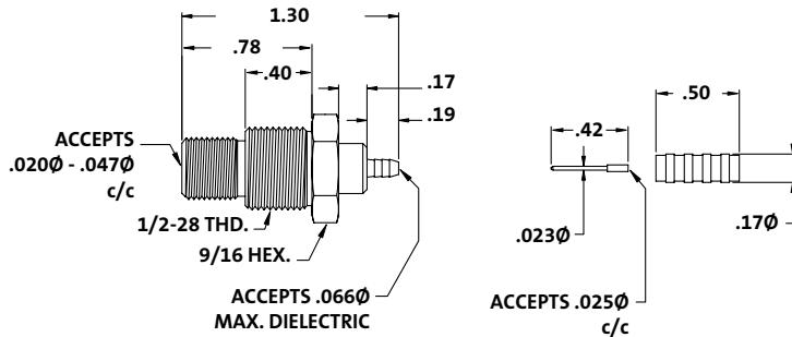
RG-179B/U 1/2" Thread Double Braided Female Coax Connector
