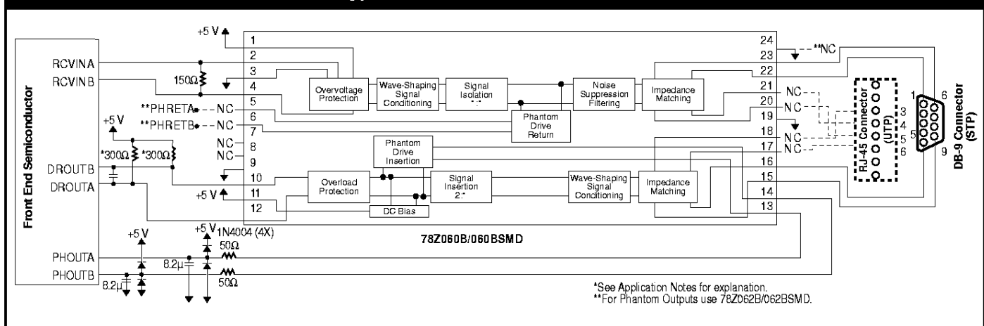
Typical Circuit with STP/UTP Node
