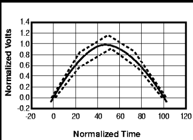
16 Mbps Binary Zeros
