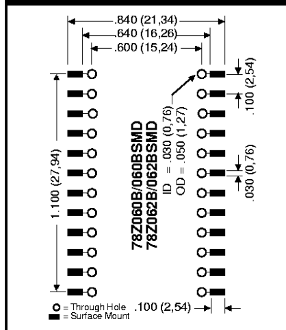
Pad Layout
