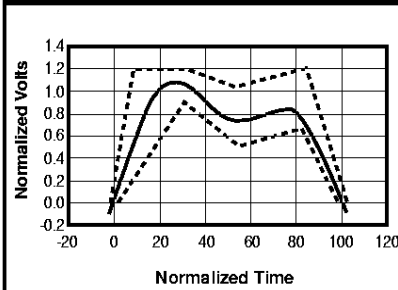
16 Mbps Binary Ones
