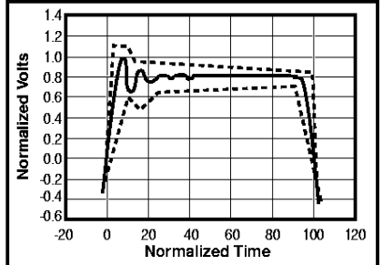
16 Mbps Start Delimeter
