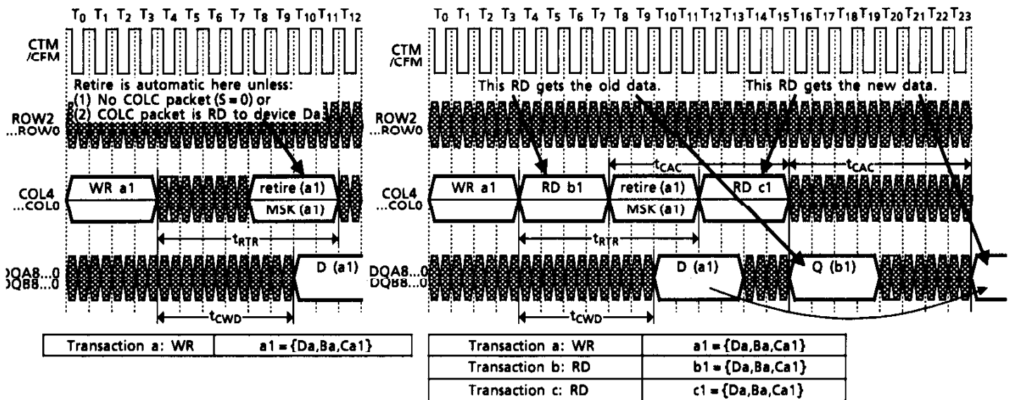
Figure 19. Normal Retire (left) and Retire/Read Ordering (right)
