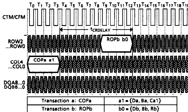
Figure 11. COL-to-ROW Packet Interaction Timing
