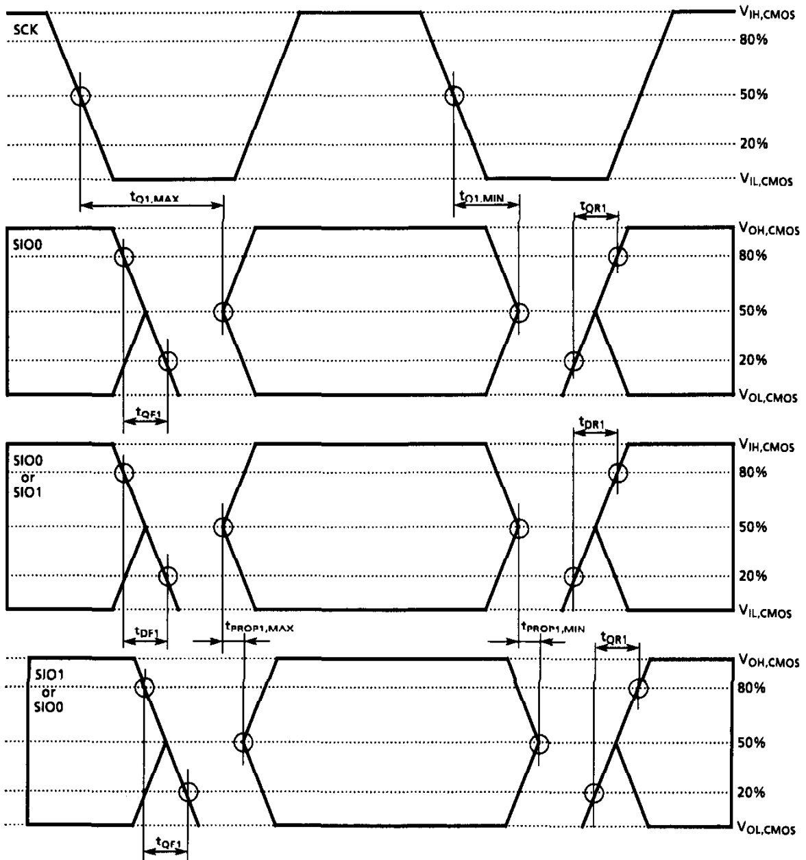
Figure 47. CMOS Timing -Data Signals for Transmit
