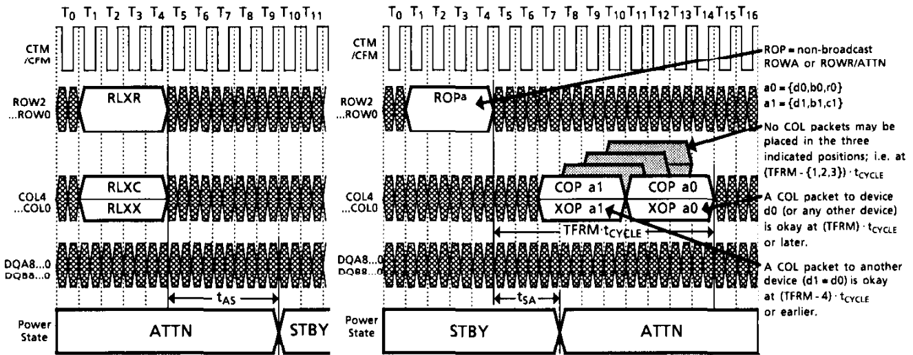
Figure 35. STBY Entry (left) and STBY Exit (right)
