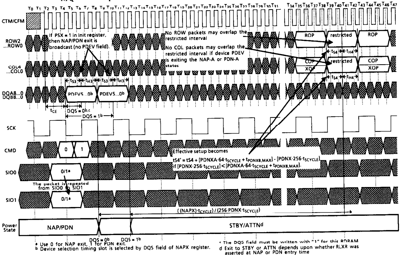
Figure 37. NAP and PDN Exit
