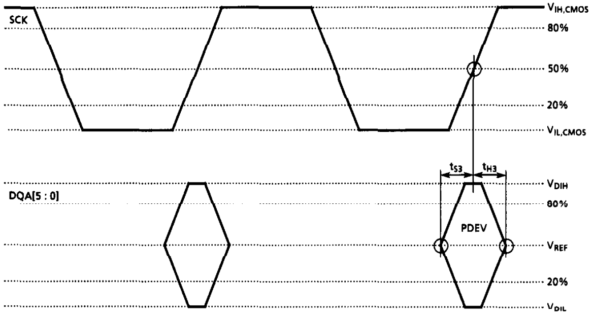
Figure 46. CMOS Timing -Device Address for NAP or PDN Exit
