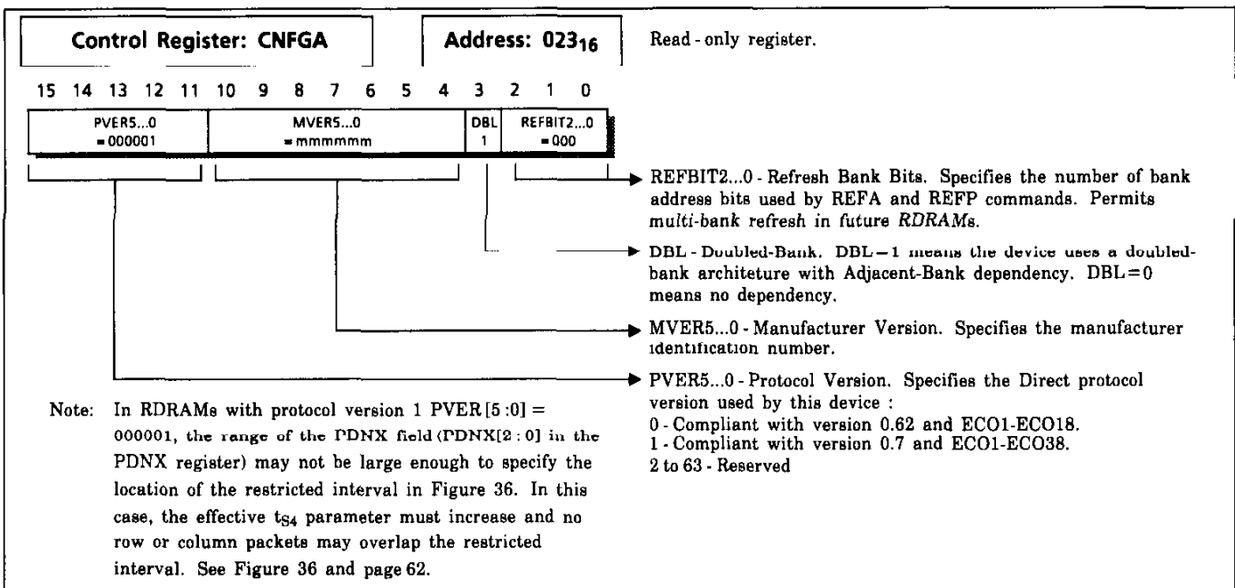
Figure 29. Control Registers
