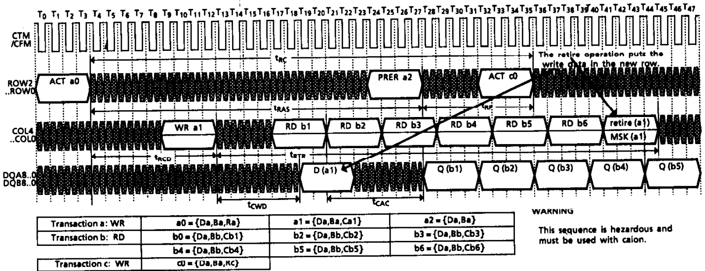
Figure 21. Retire Held off by Reads to Same Device, Write Buffer Retired to New Row
