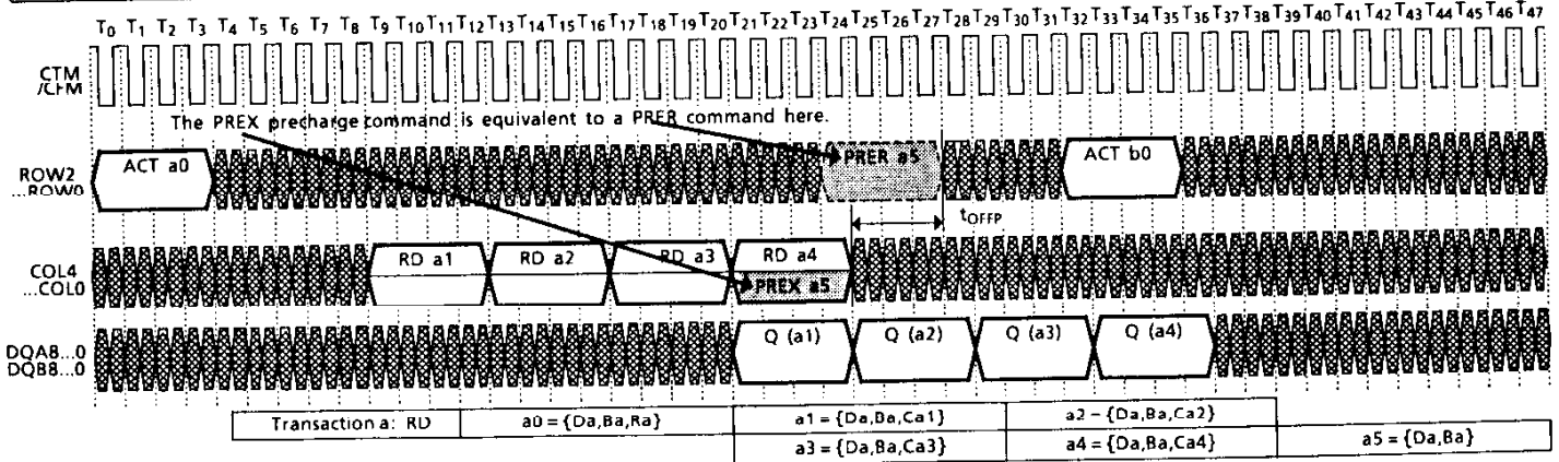
Figure 16. Offsets for Alternative Precharge Mechanisms
