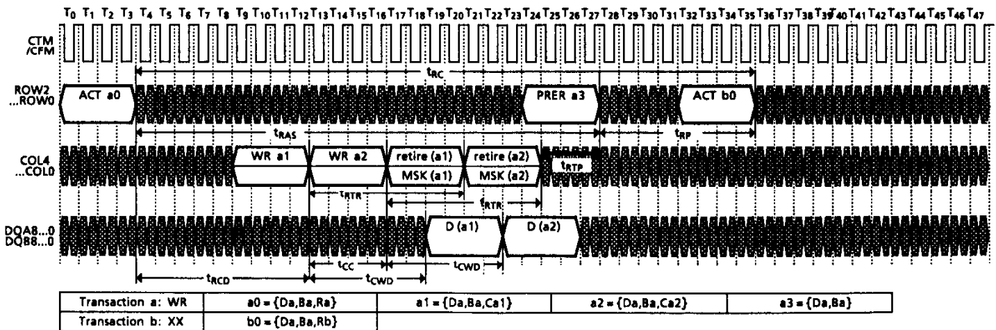
Figure 18. Write Transaction Example
