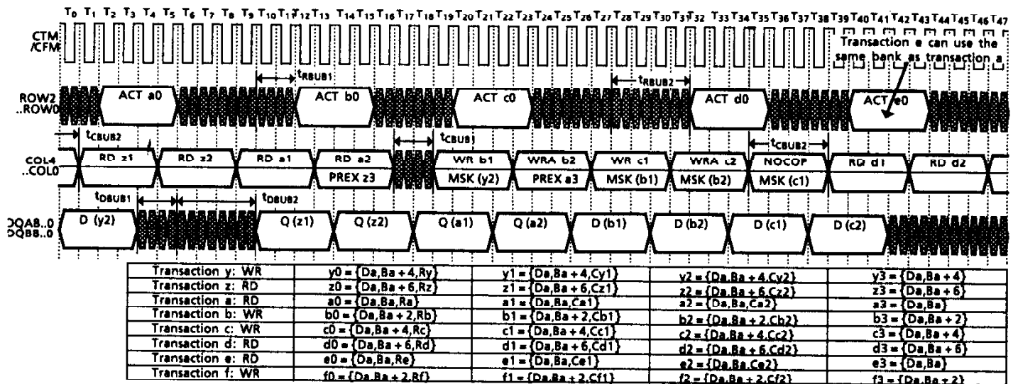
Figure 24. Interleaved RRWW Sequence with Two Dualocts Data Length
