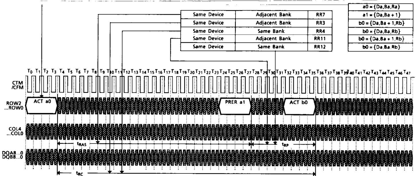
Figure 12. Row Packet Example
