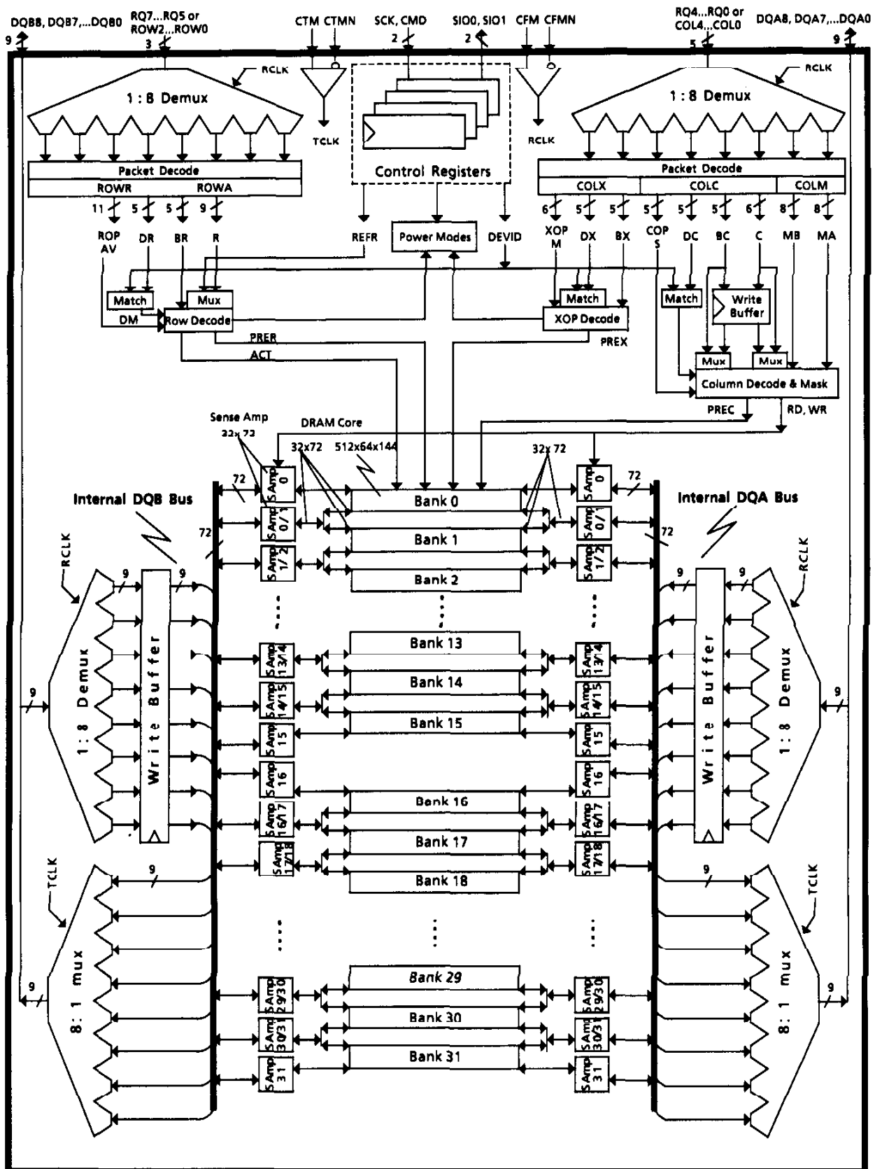
Figure 4. 144-Mbit Direct RDRAM Block Diagram
