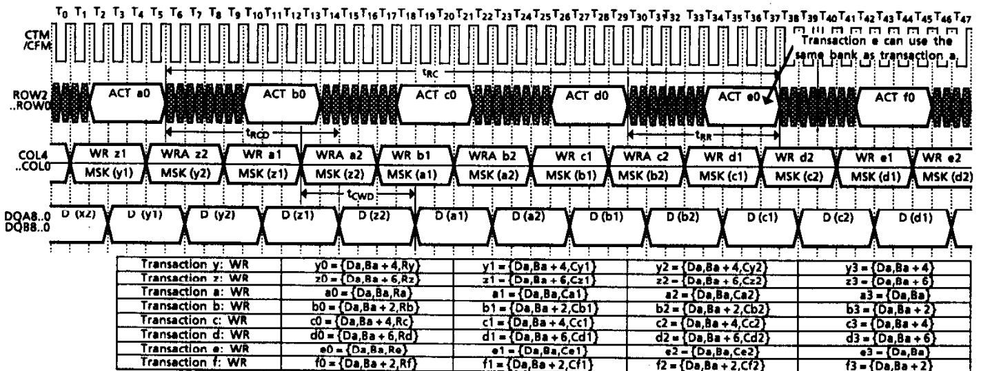
Figure 22. Interleaved Write Transaction with Two Dualocts Data Length
