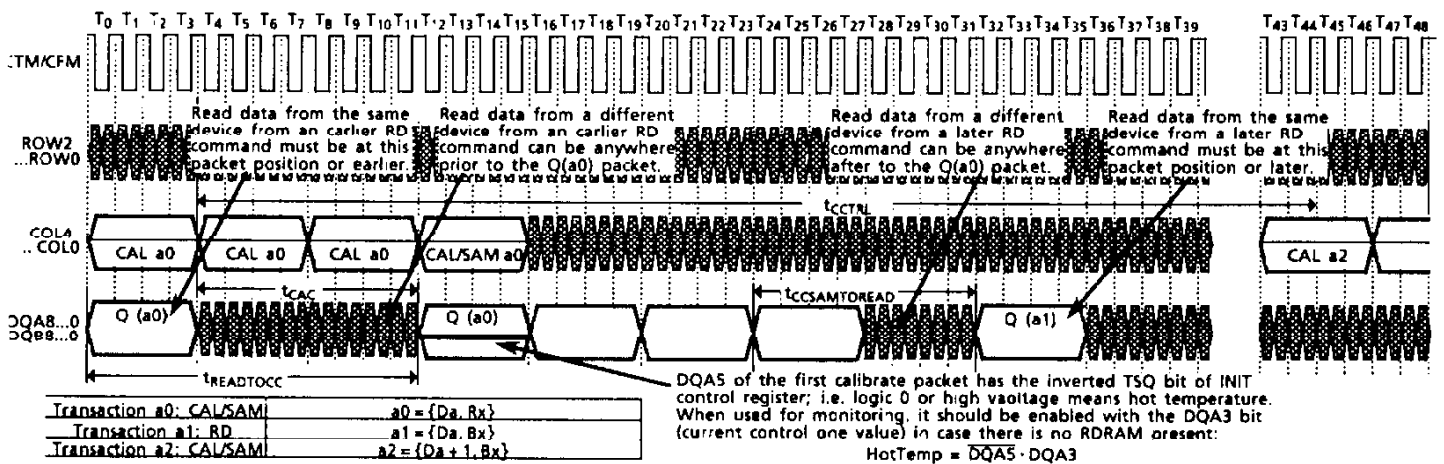
Figure 40. Current Control CAL/SAM transaction Example
