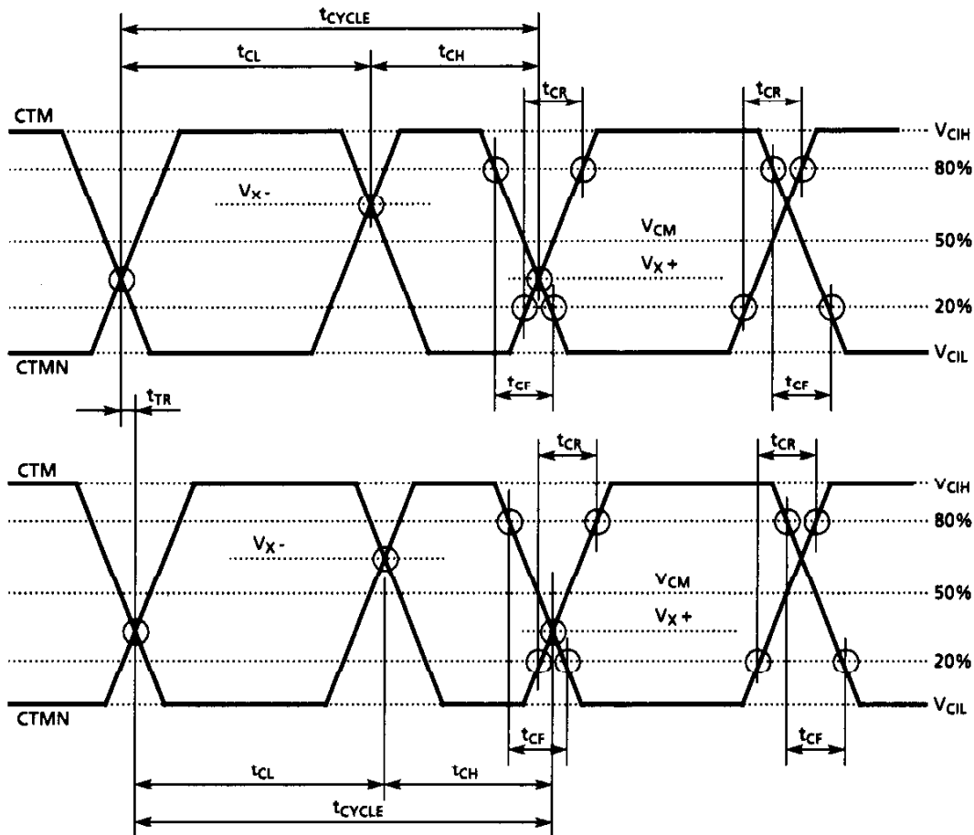
Figure 42. RSL Timing -Clock Signals
