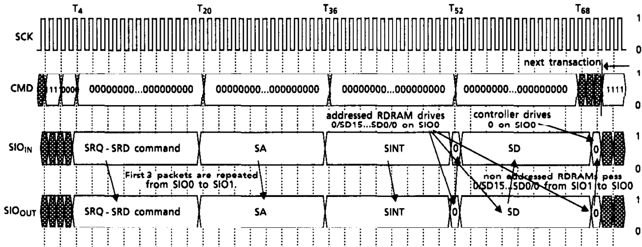
Figure 26. Serial Read (SRD) Transaction to Control Register
