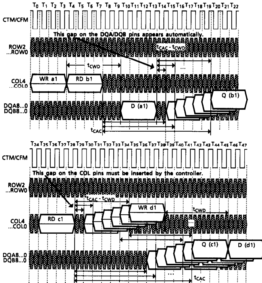
Figure 6. Read(Q) and Write (D) Data Packets - Timings for t_{CAC} = 7, 8, 9, 10, 11 or 12 t_{CYCLE}
