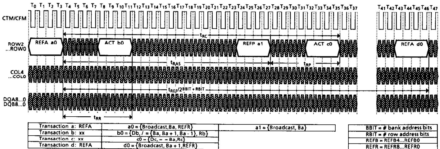
Figure 39. REFA/REFP Refresh Transaction Example
