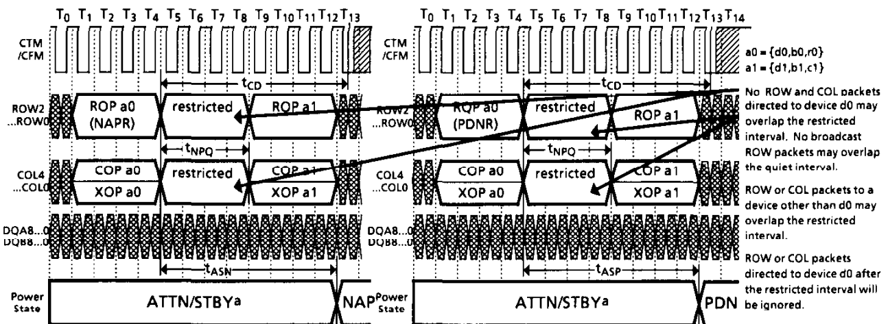
Figure 36. NAP Entry (left) and PDN Entry (right)
