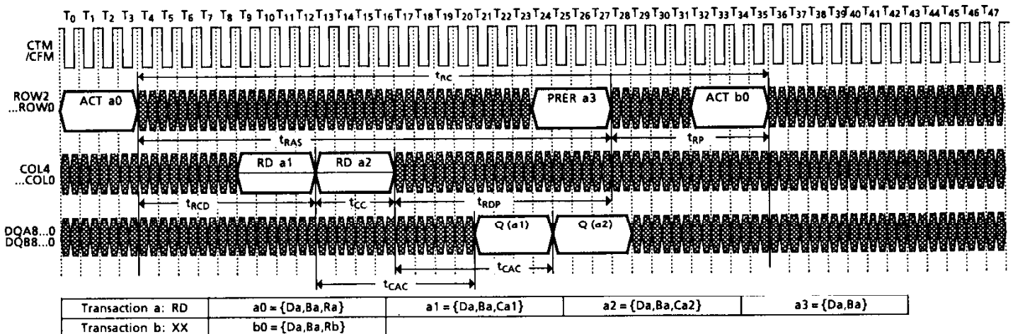
Figure 17. Read Transaction Example
