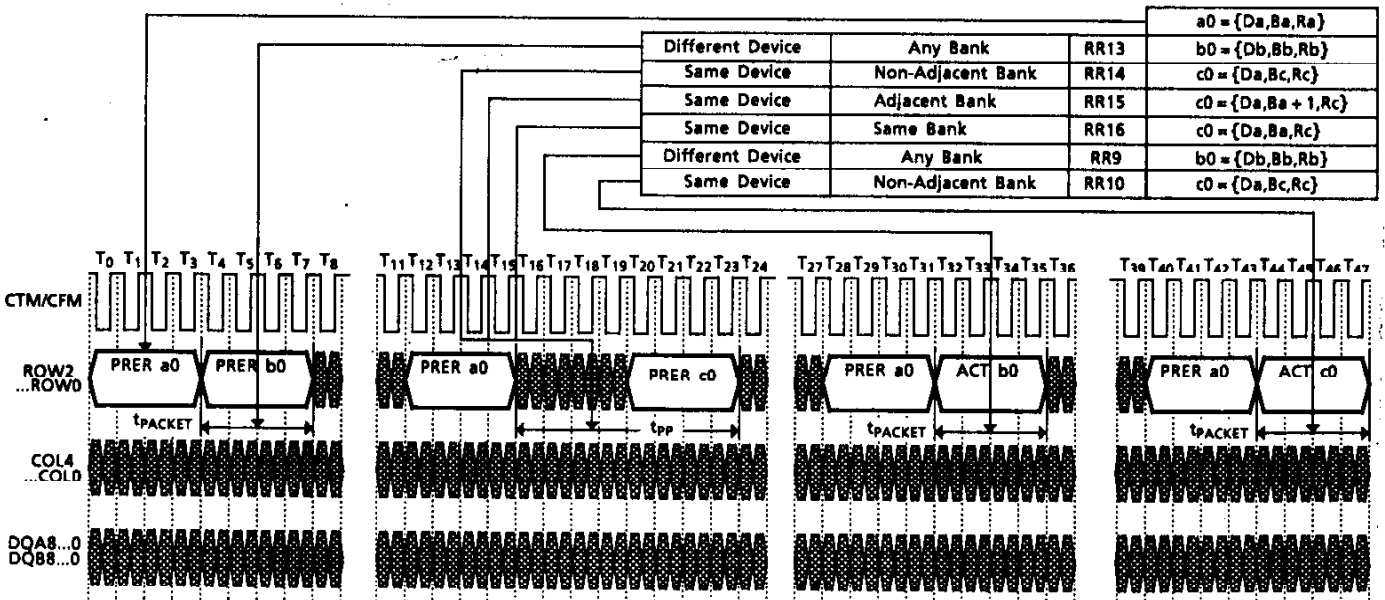
Figure 14. Row Packet Examples
