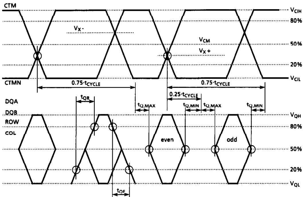
Figure 44. RSL Timing -Data Signals for Transmit
