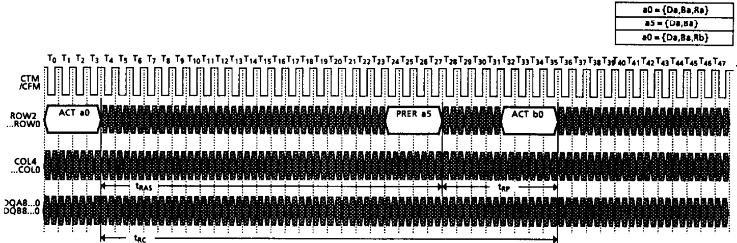
Figure 15. Precharge with PRER Command in ROWR Packet
