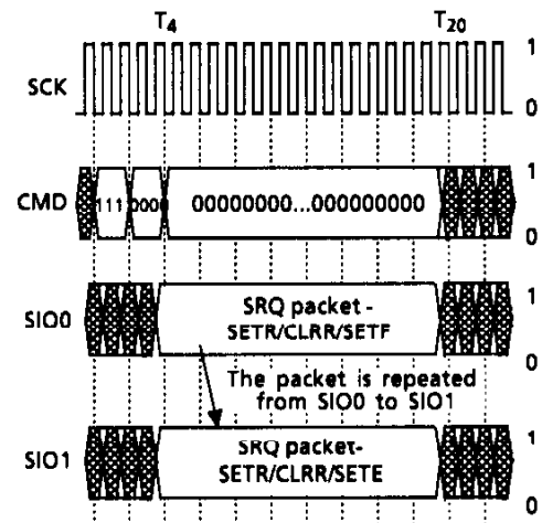
Figure 27. SETR, CLRR, SETF Transaction
