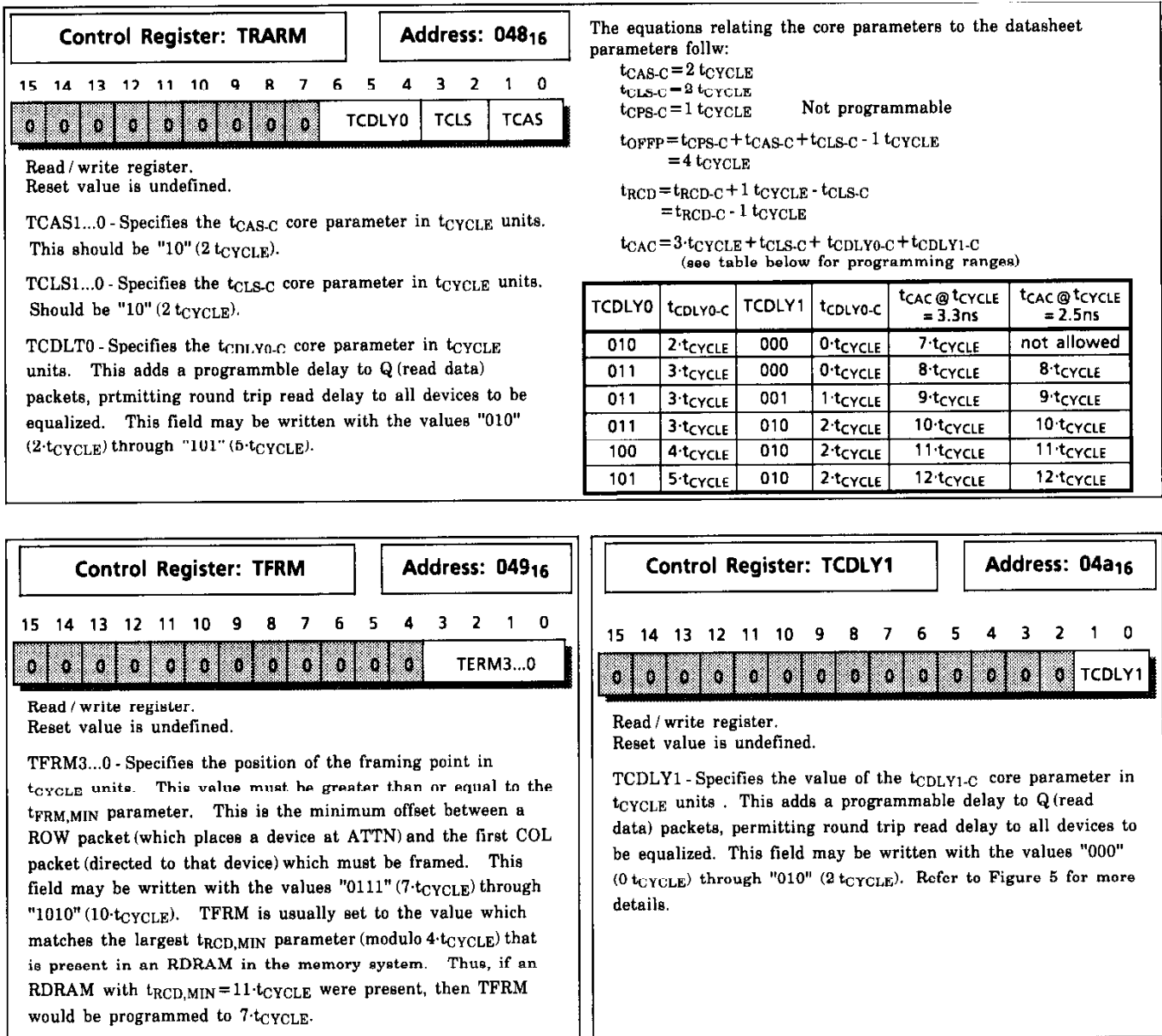
Figure 32. Control Registers
