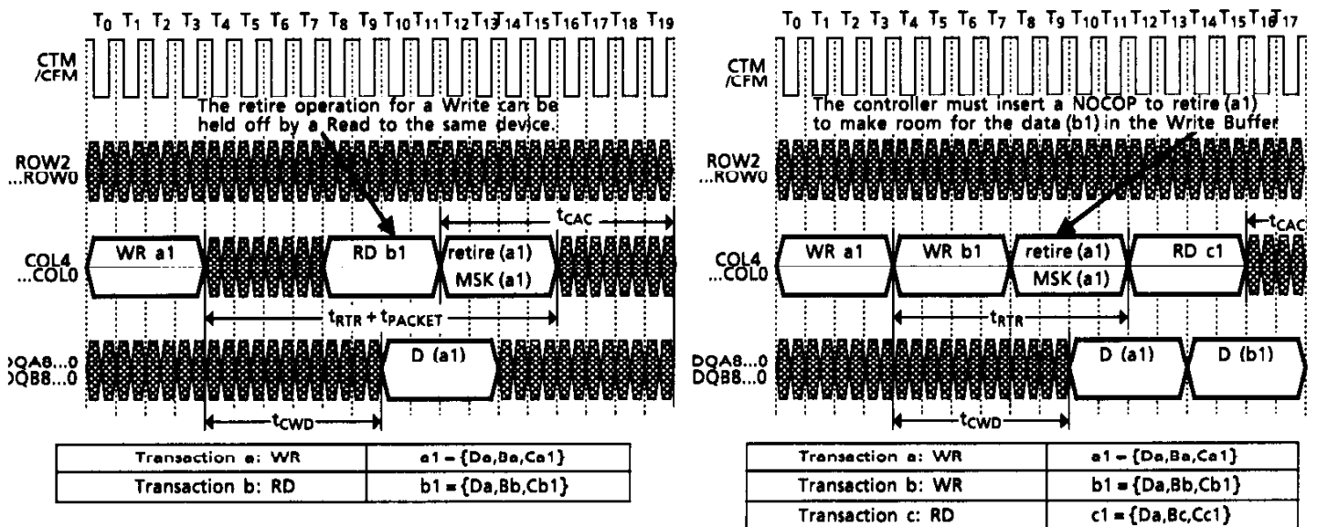
Figure 20. Retire Held off by Read (left) and Controller Forcing WWR Gap (right)
