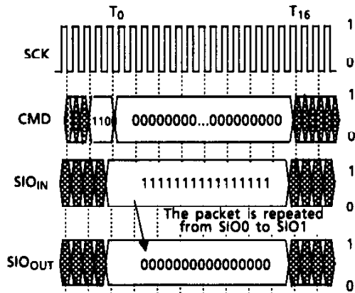
Figure 28. SIO Reset Sequence
