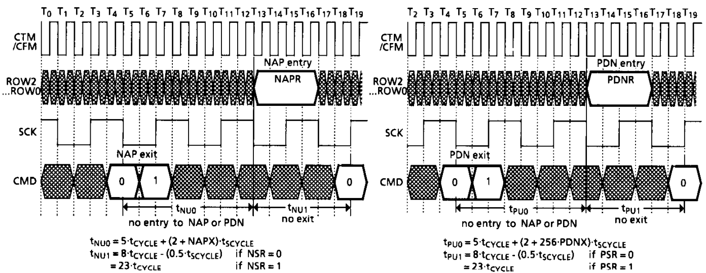
Figure 38. NAP Entry / Exit Windows (left) and PDN Entry / Exit Windows (right)
