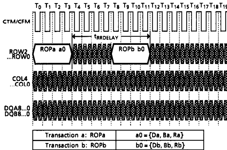
Figure 8. ROW-to-ROW Packet Interaction -Timing
