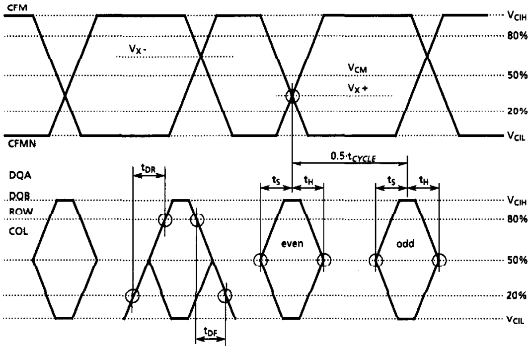
Figure 43. RSL Timing - Data Signals for Receive
