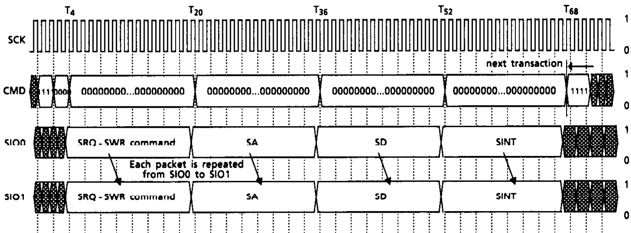
Figure 25. Serial Write (SWR) Transaction to Control Register
