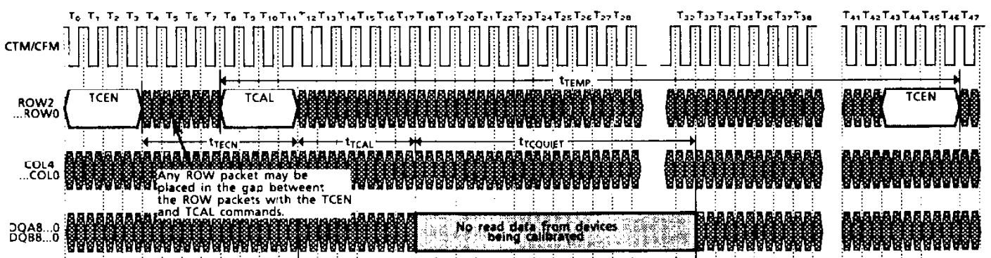
Figure 41. Temperature Calibration (TCEN-TCAL) Transitions to RDRAM
