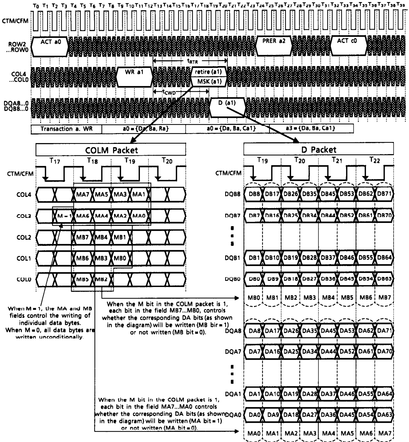
Figure 7. Mapping Between COLM Packet and D Packet for WR Command
