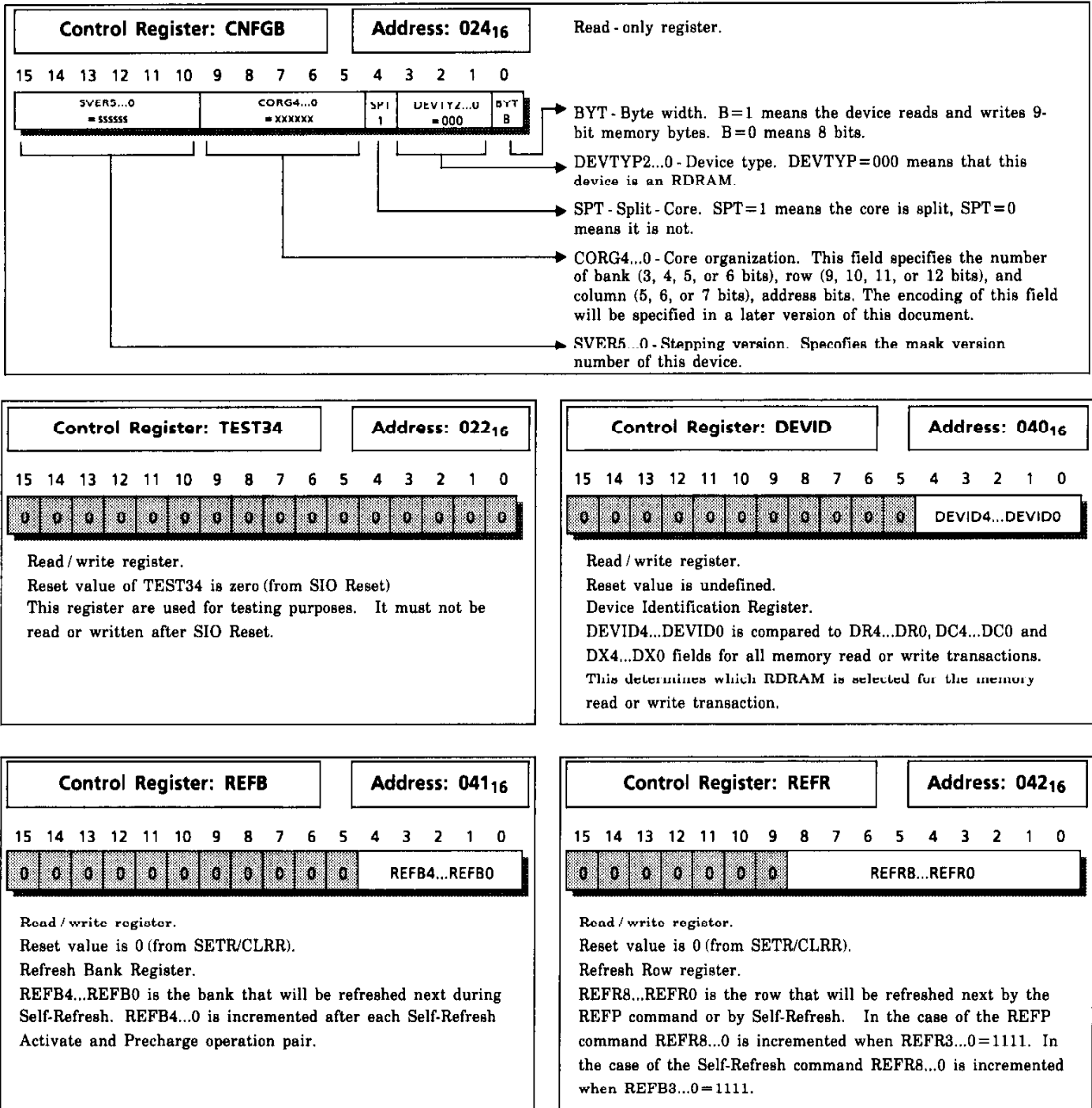
Figure 30. Control Registers
