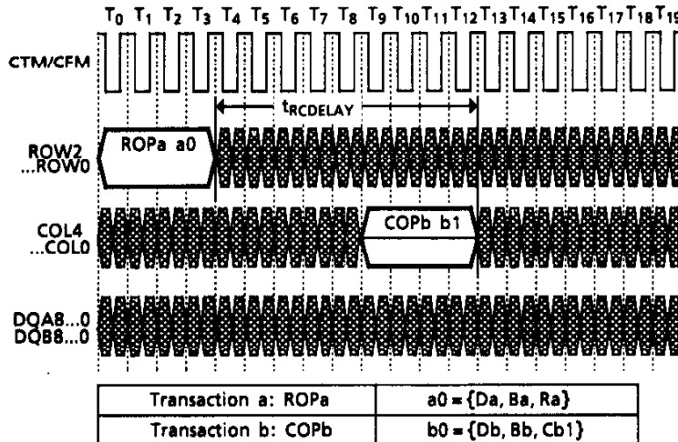
Figure 9. ROW-to-COL Packet Interaction Timing
