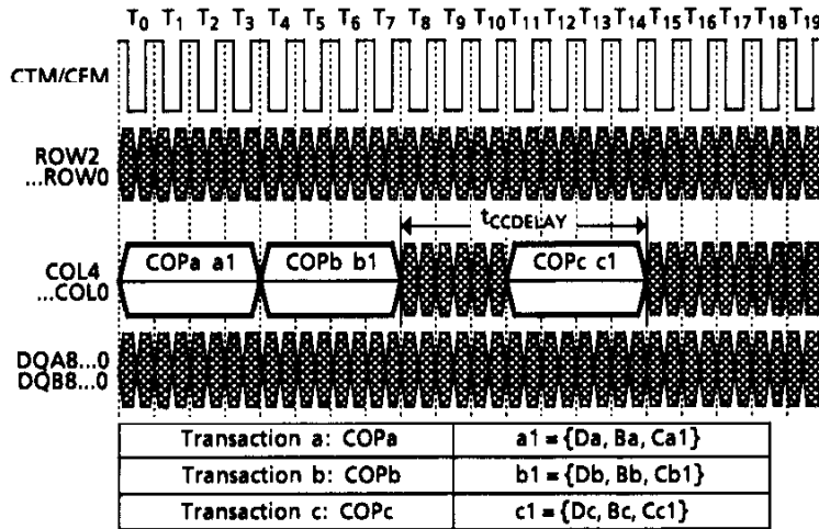
Figure 10. COL-to-COL Packet Interaction Timing
