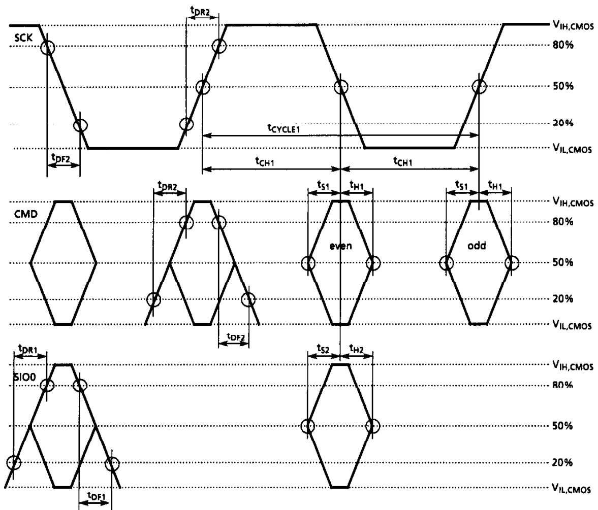
Figure 45. CMOS Timing -Data Signals for Receive
