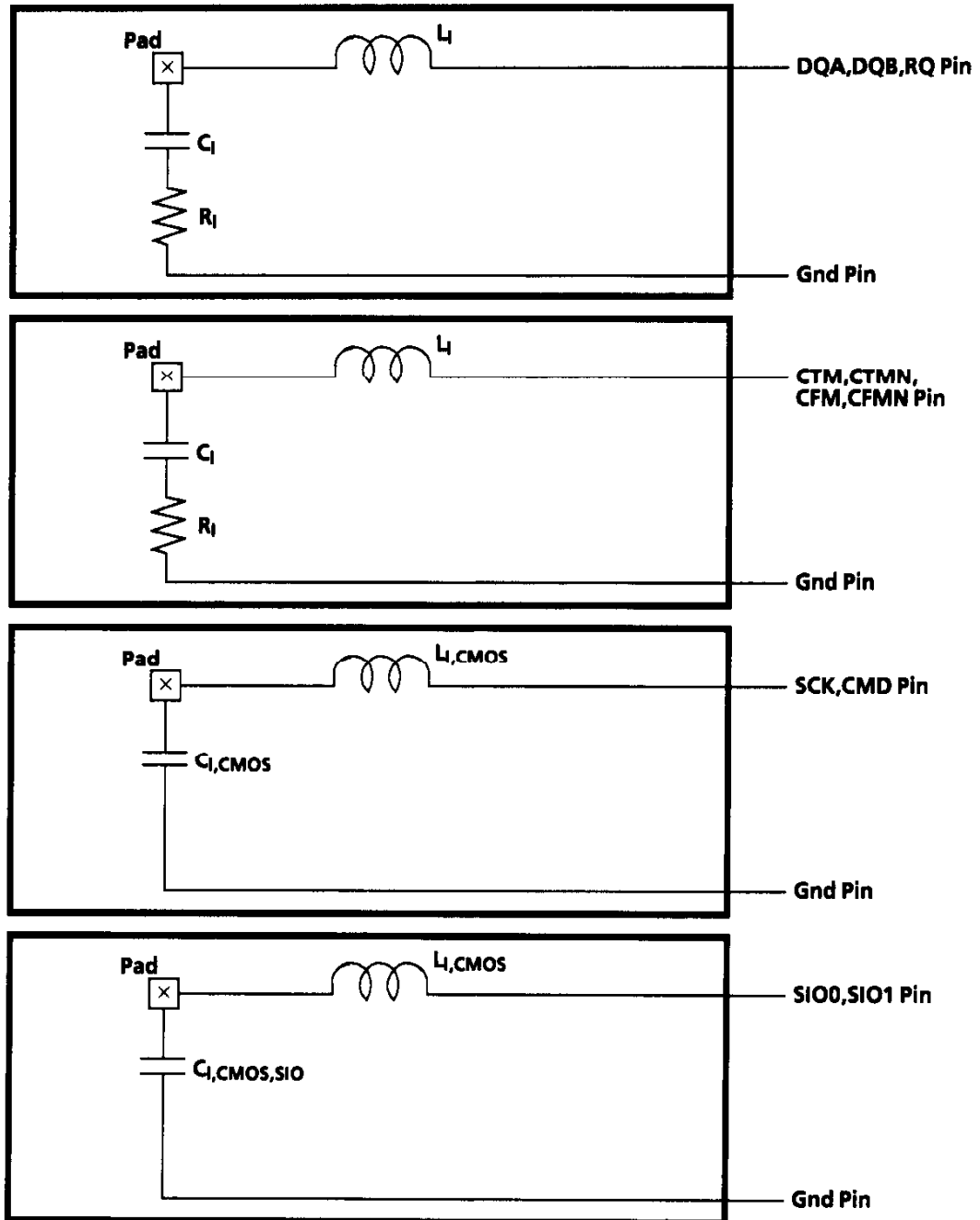
Figure 49. Equivalent Load Circuit for RSL Pins
