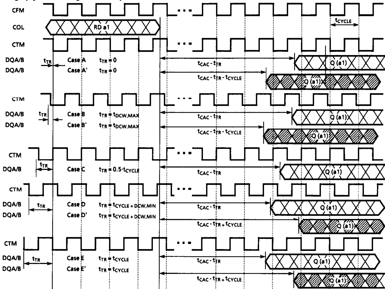
Figure 48. RSL Transmit -Crossing Read Domains
