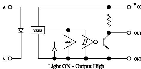
OPL482/492 Inverter with Pull-Up Resistor
