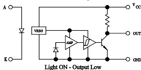
OPL480/490 Buffer with Pull-Up Resistor
