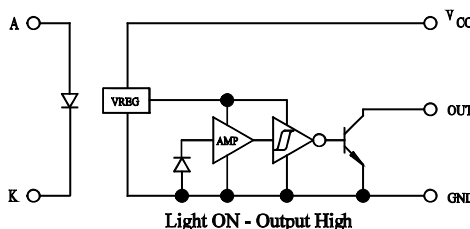
OPL483/493 Inverter / Open Collector
