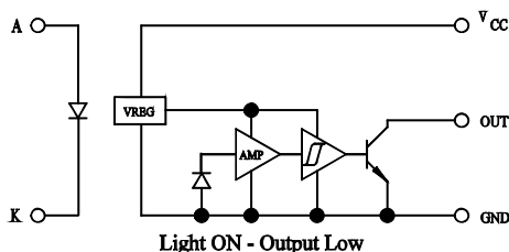
OPL481/491 Buffer / Open Collector
