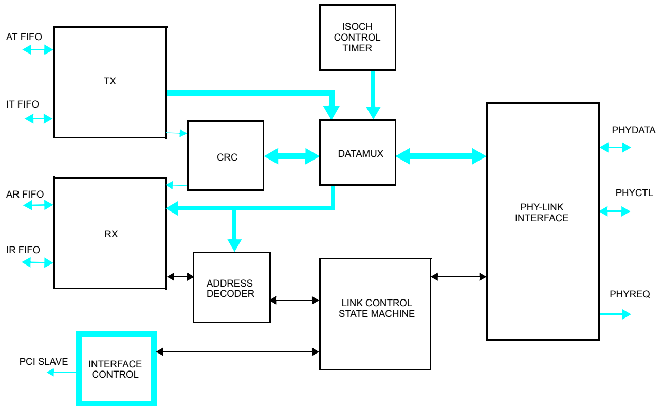
Figure 4. Link Core Block Diagram
